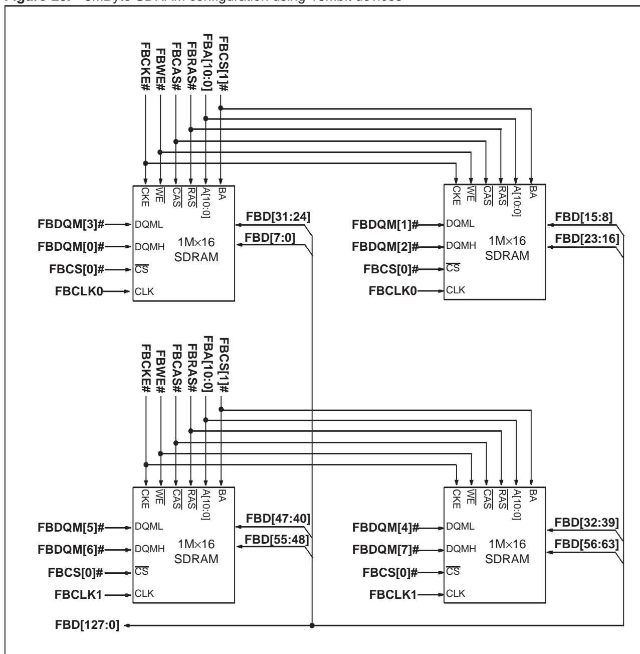
Figure 28. 8MByte SDRAM configuration using 16Mbit devices
