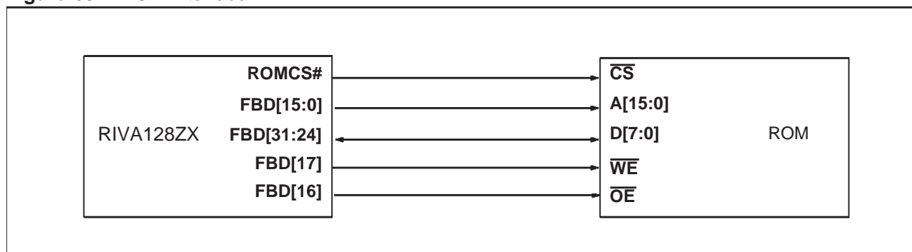
Figure 63. ROM interface
