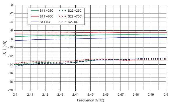
Figure 18: S-Parameter Data S11 and S22, 3.3 V
