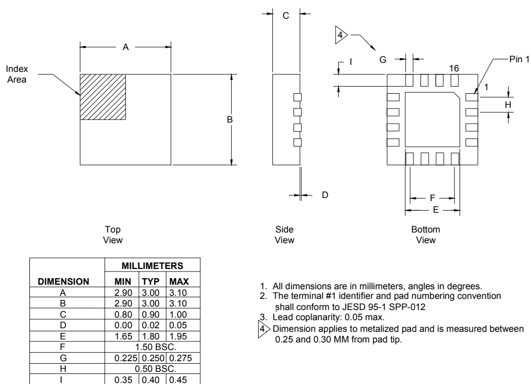
Figure 20: Package Outline
