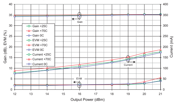
Figure 4: Gain, Current, EVM vs. Output Power at 2.437 GHz, 3.3 V (IEEE 802.11g @ 54 Mbps)
