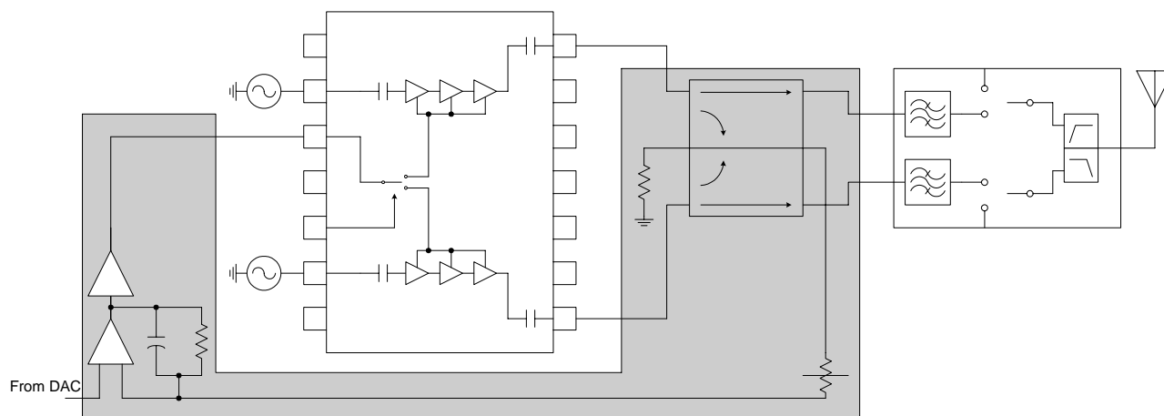
Traditional Triple-Band PA
