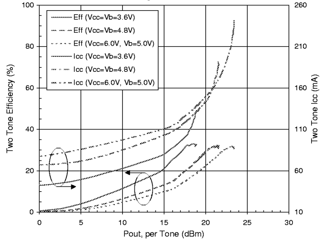
Two Tone Efficiency and Icc vs. Pout, 915 MHz
