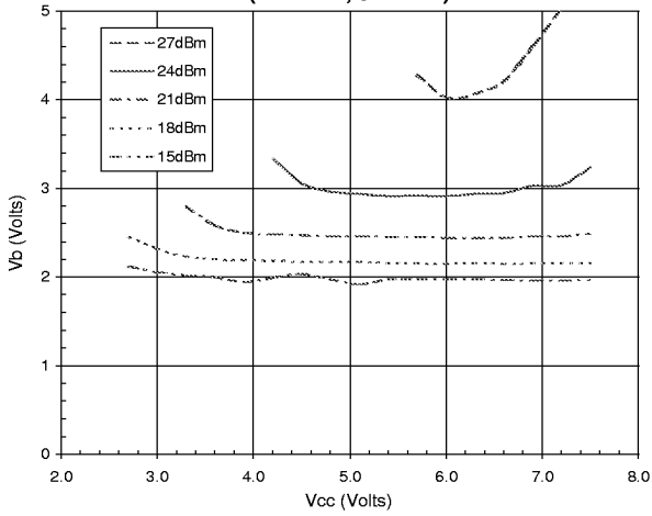
Vb Required to Achieve Specific Pout (Vb<5.0 V, 915 MHz)
