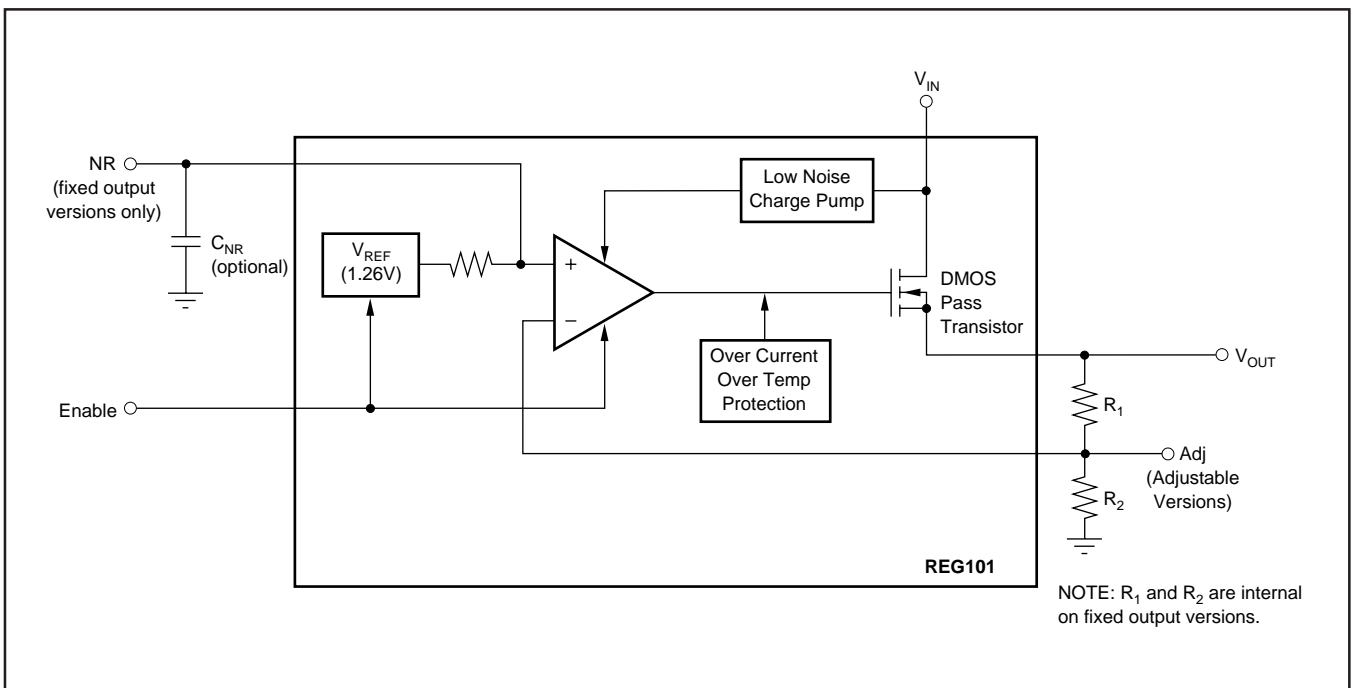
FIGURE 4. Block Diagram.
