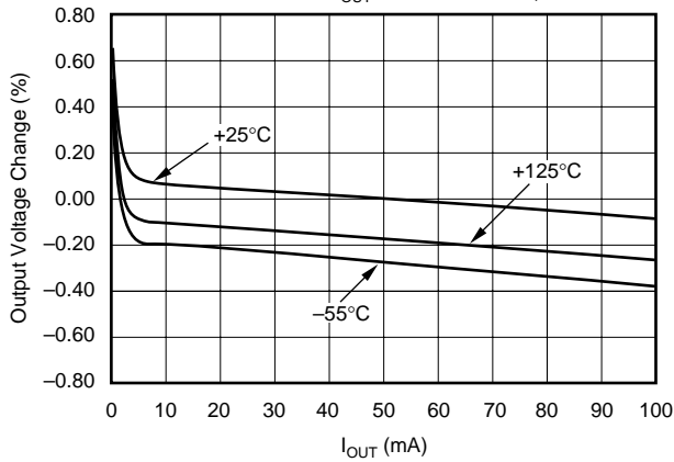
OUTPUT VOLTAGE CHANGE vs I_{\text{OUT}} (V_{\text{IN}} = V_{\text{OUT}} + 1\text{V}, \text{Output Voltage \% Change} Referred to I_{\text{OUT}} = 50\text{mA} at +25^\circ\text{C} )
