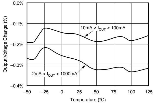
LOAD REGULATION vs TEMPERATURE (V_{\text{IN}} = V_{\text{OUT}} + 1\text{V})
