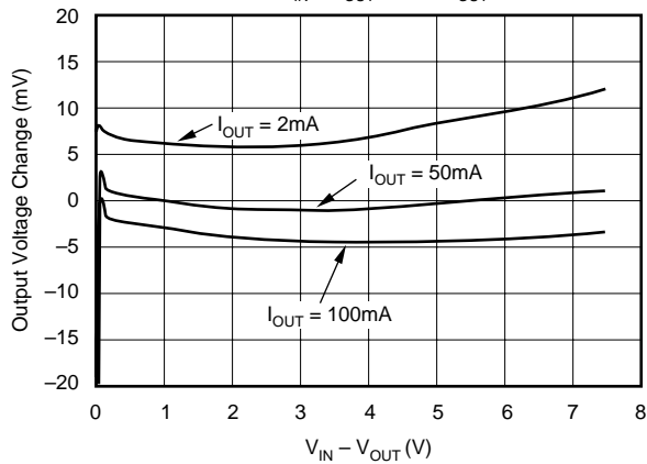
LINE REGULATION (Referred to V_{\text{IN}} = V_{\text{OUT}} + 1\text{V} at I_{\text{OUT}} = 50\text{mA} )
