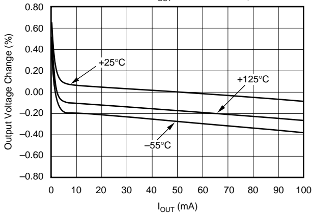
OUTPUT VOLTAGE CHANGE vs I_{\text{OUT}} (V_{\text{IN}} = V_{\text{OUT}} + 1\text{V} , Output Voltage % Change Referred to I_{\text{OUT}} = 50\text{mA} at +25^\circ\text{C} )
