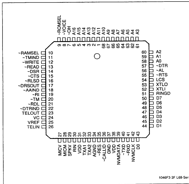
Figure 5. Modem Pin Signals - 68-Pin PLCC - Serial DTE Interface
