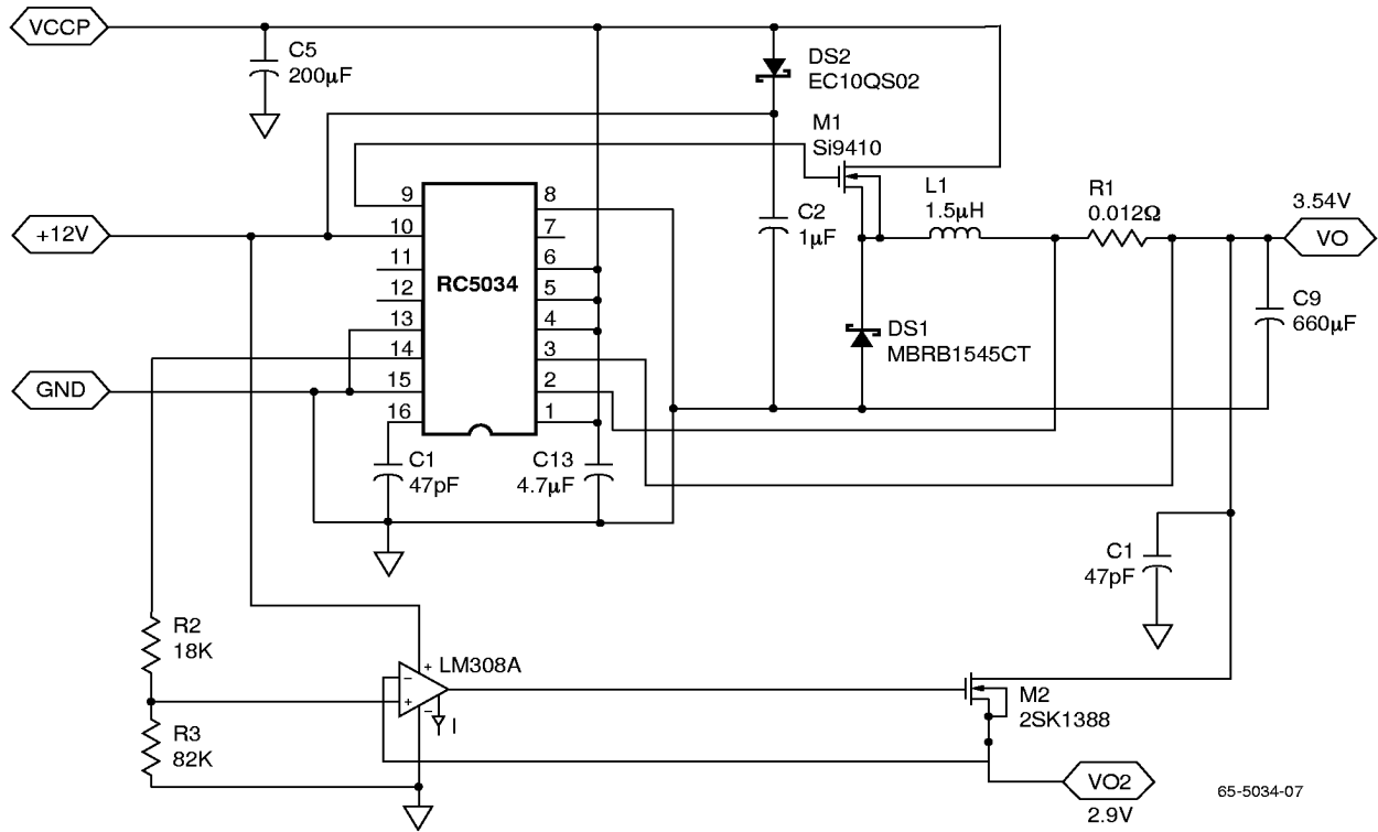
Figure 3. Dual Regulator Applications Circuit
