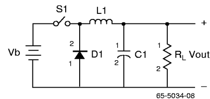
Figure 4. Simple Buck DC-DC Converter
