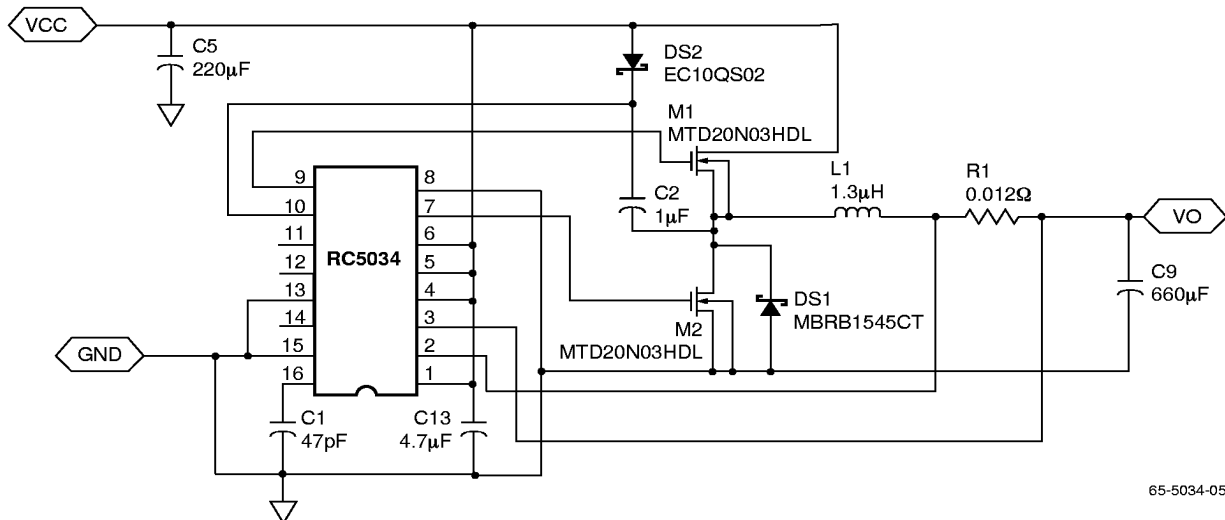
Figure 1. Synchronous 7A Schematic
