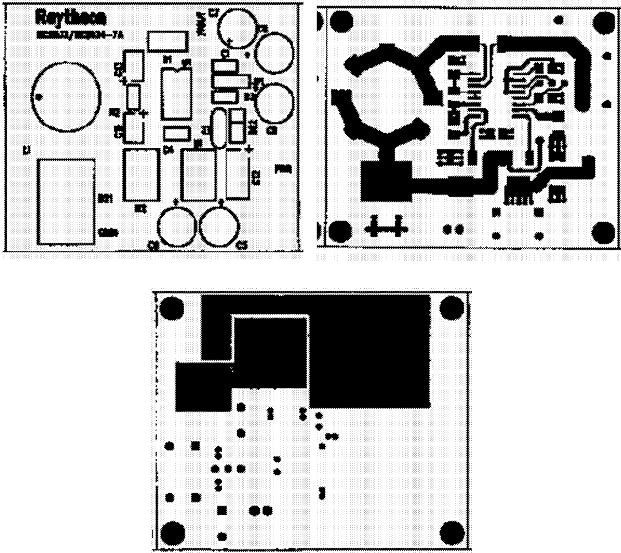
Figure 5. Sample PCB Layout
