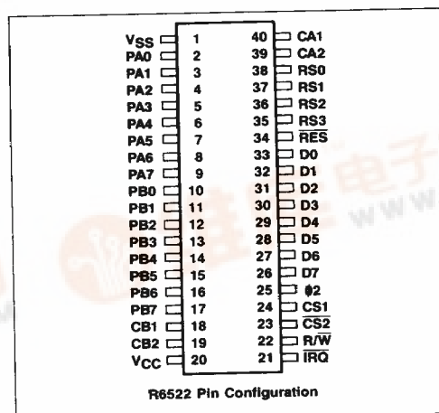
Figure 1. R6522 Pin Assignments
