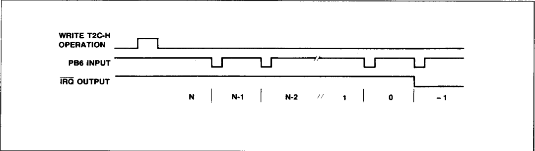
Figure 19. Timer 2 Pulse Counting Mode
