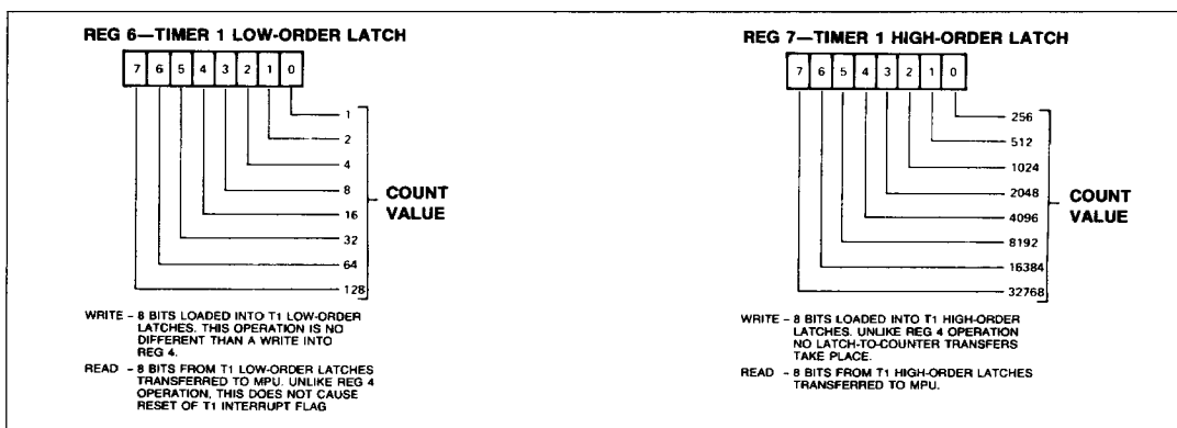
Figure 12. Timer 1 (T1) Latch Registers
