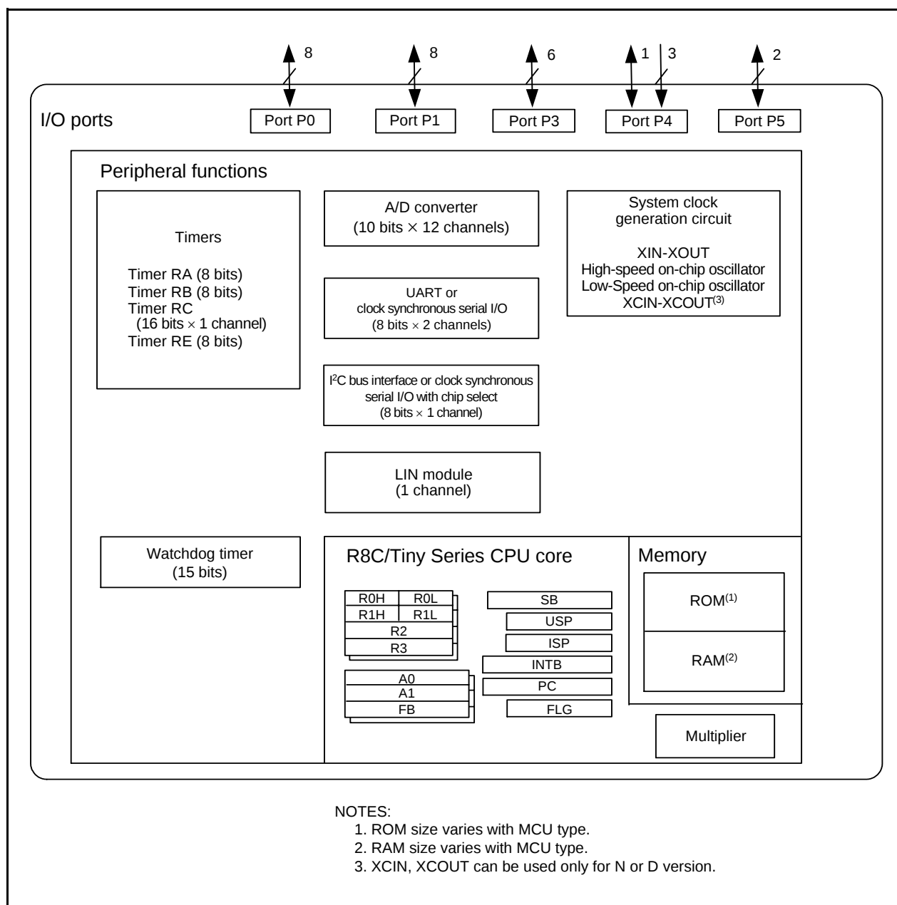
Figure 1.1 Block Diagram
