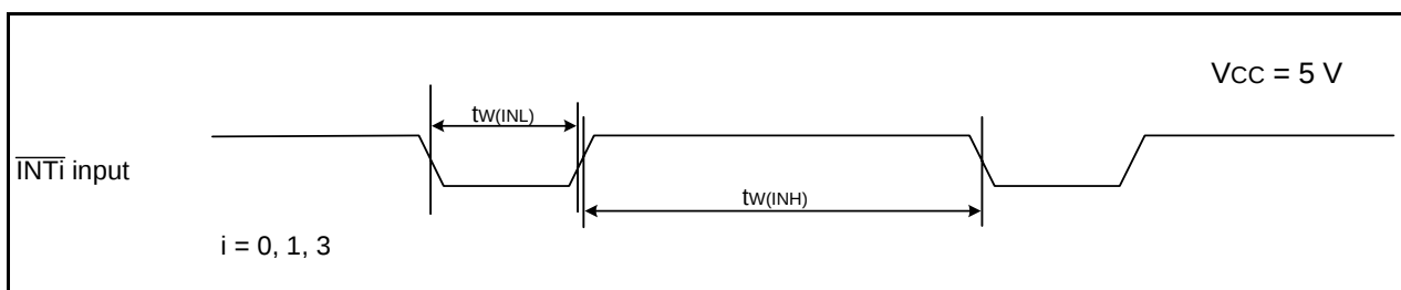
Figure 5.30 External Interrupt \overline{INTi} Input Timing Diagram when Vcc = 5 V
