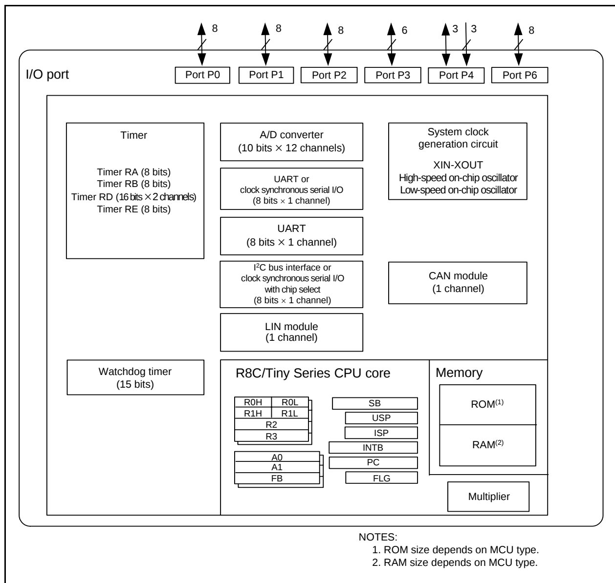
Figure 1.1 Block Diagram
