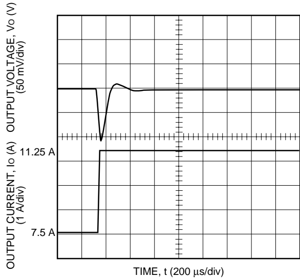
Figure 9. Typical QW050F1 Transient Response to Step Increase in Load from 50% to 75% of I_{o,max} at Room Temperature and 54 Vdc Input (Waveform Averaged to Eliminate Ripple Component.)
