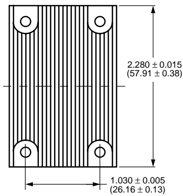
Figure 33. Longitudinal Heat Sink
