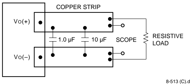
Figure 13. Input Reflected-Ripple Test Setup
