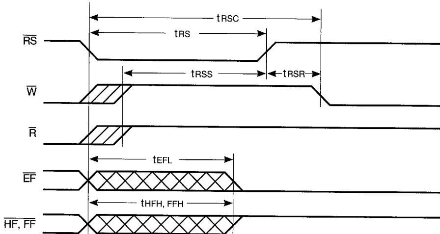
FIGURE 5. RESET TIMING
