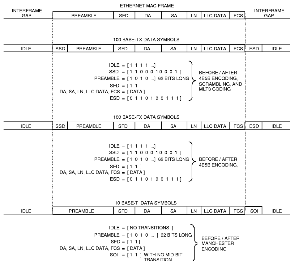
Figure 2. Frame Format
