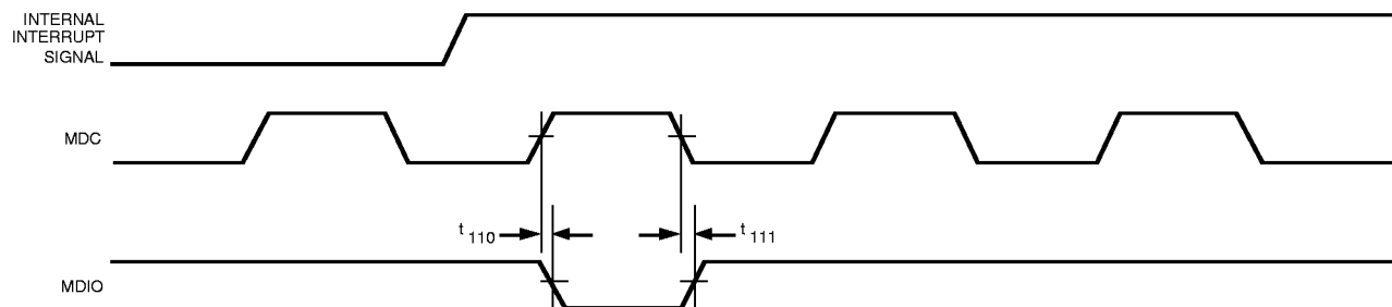
Figure 32. MDIO Interrupt Pulse Timing
