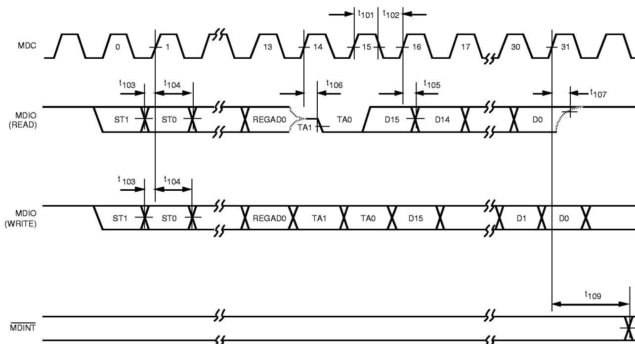
Figure 31. MI Serial Port Timing
