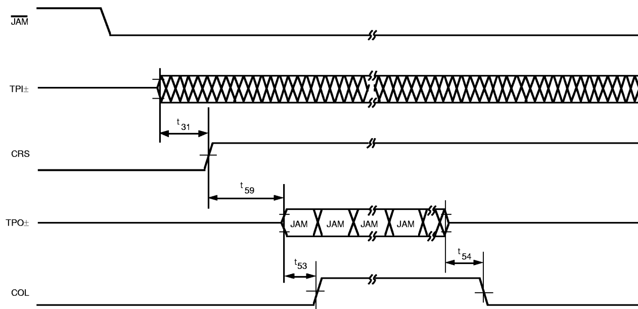
Figure 26. Jam Timing
