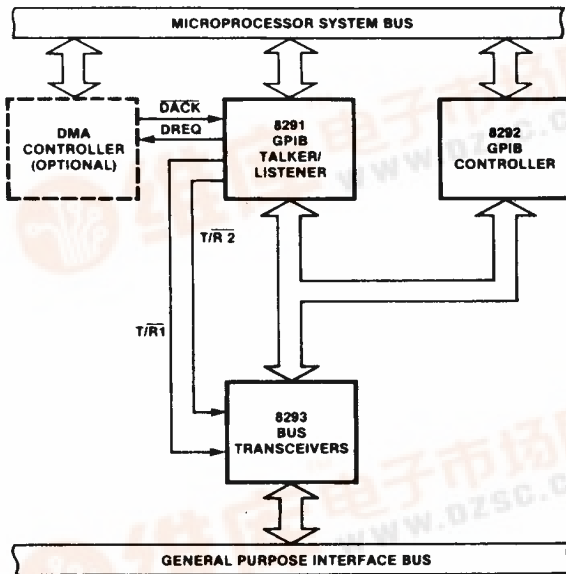
Figure 1. 8291, 8292 Block Diagram
