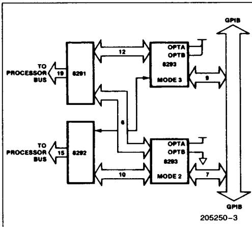
Figure 3. Talker/Listener/Controller Configuration
