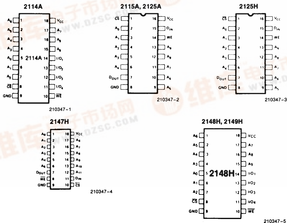
Pin Configuration
