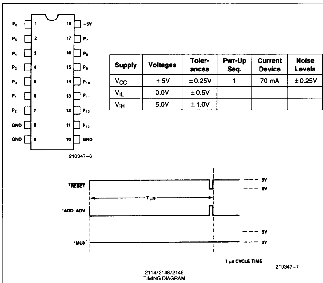
Figure 1. 2114A, 2148H, 2149H Burn-In Configuration
