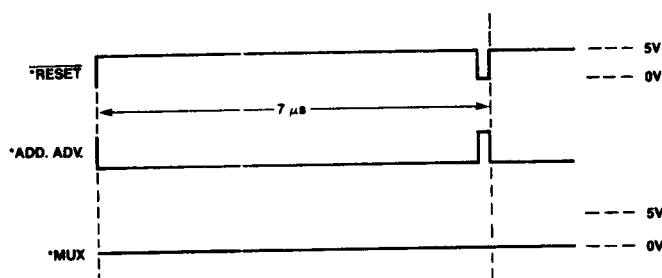
Figure 2. 2115, 2125 Burn-In Configuration
