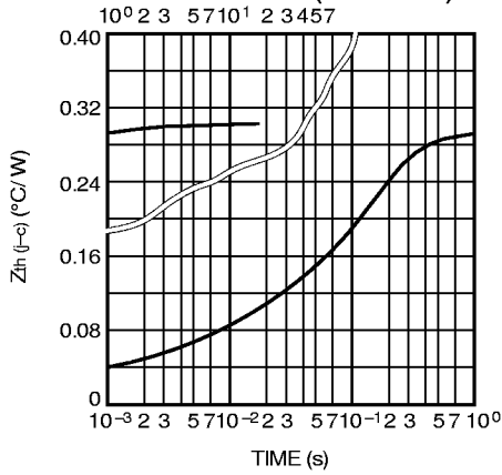
TRANSIENT THERMAL IMPEDANCE CHARACTERISTIC (DIODE PART)
