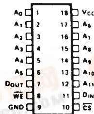
Figure 2. Pin Configuration
