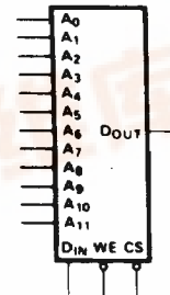
Figure 3. Logic Symbol
