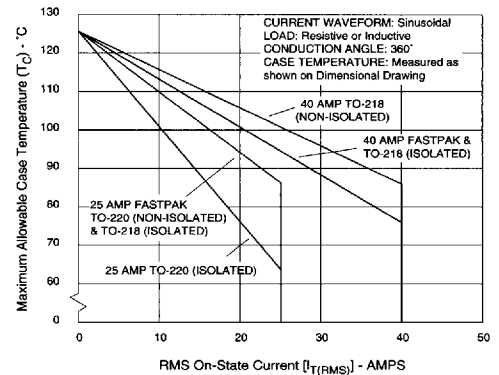
Figure 1F — Maximum Allowable Case Temperature vs On-State Current
