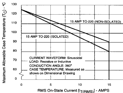
Figure 1E — Maximum Allowable Case Temperature vs On-State Current
