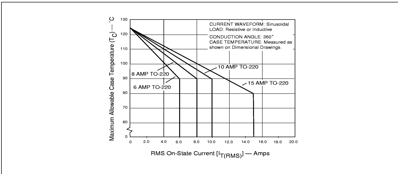
Figure 3.8 Maximum Allowable Case Temperature vs On-State Current (6-15 Amp)
