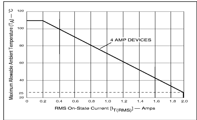
Figure 3.6 Maximum Allowable Ambient Temperature vs On-State Current
