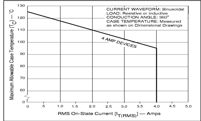
Figure 3.7 Maximum Allowable Case Temperature vs On-State Current (4 Amp)
