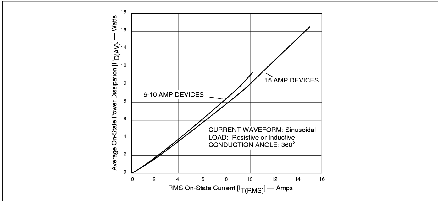
Figure 3.11 Power Dissipation (Typical) vs. On-State Current (6-10 and 15 Amp)
