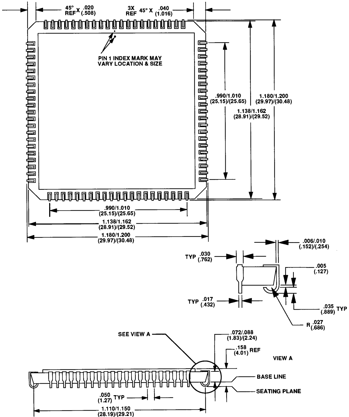
FIGURE 17. CLDCC PACKAGING
