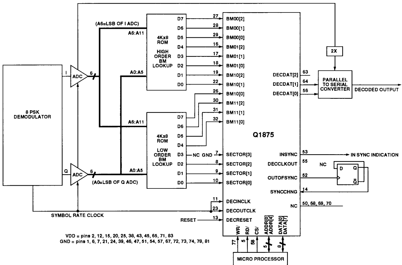
FIGURE 12. RATE 2/3 8-PSK DECODER CONFIGURATION EXAMPLE
