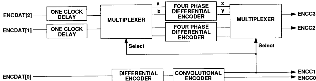
FIGURE 10. PHASE AMBIGUITY RESOLUTION ENCODER FOR 16-PSK MODULATION
