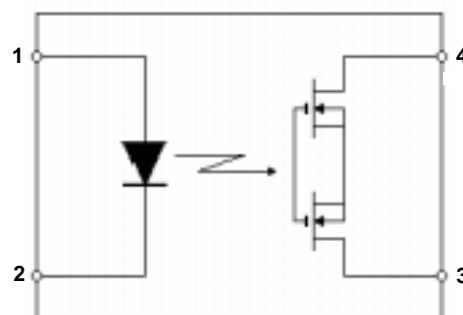
Connection Diagram
