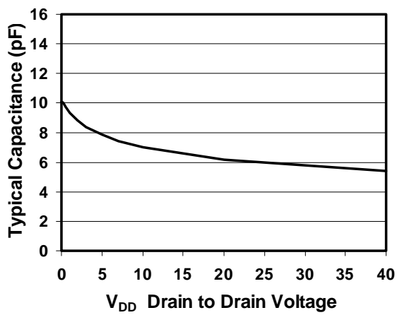
Figure 7. Output Capacitance
