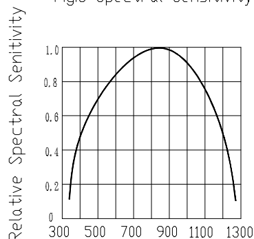
Fig.5 Spectral Sensitivity
