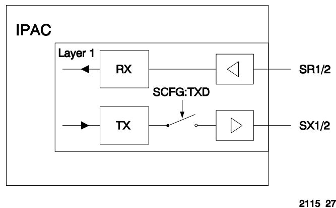
Figure 31 Disabling of S/T Transmitter
