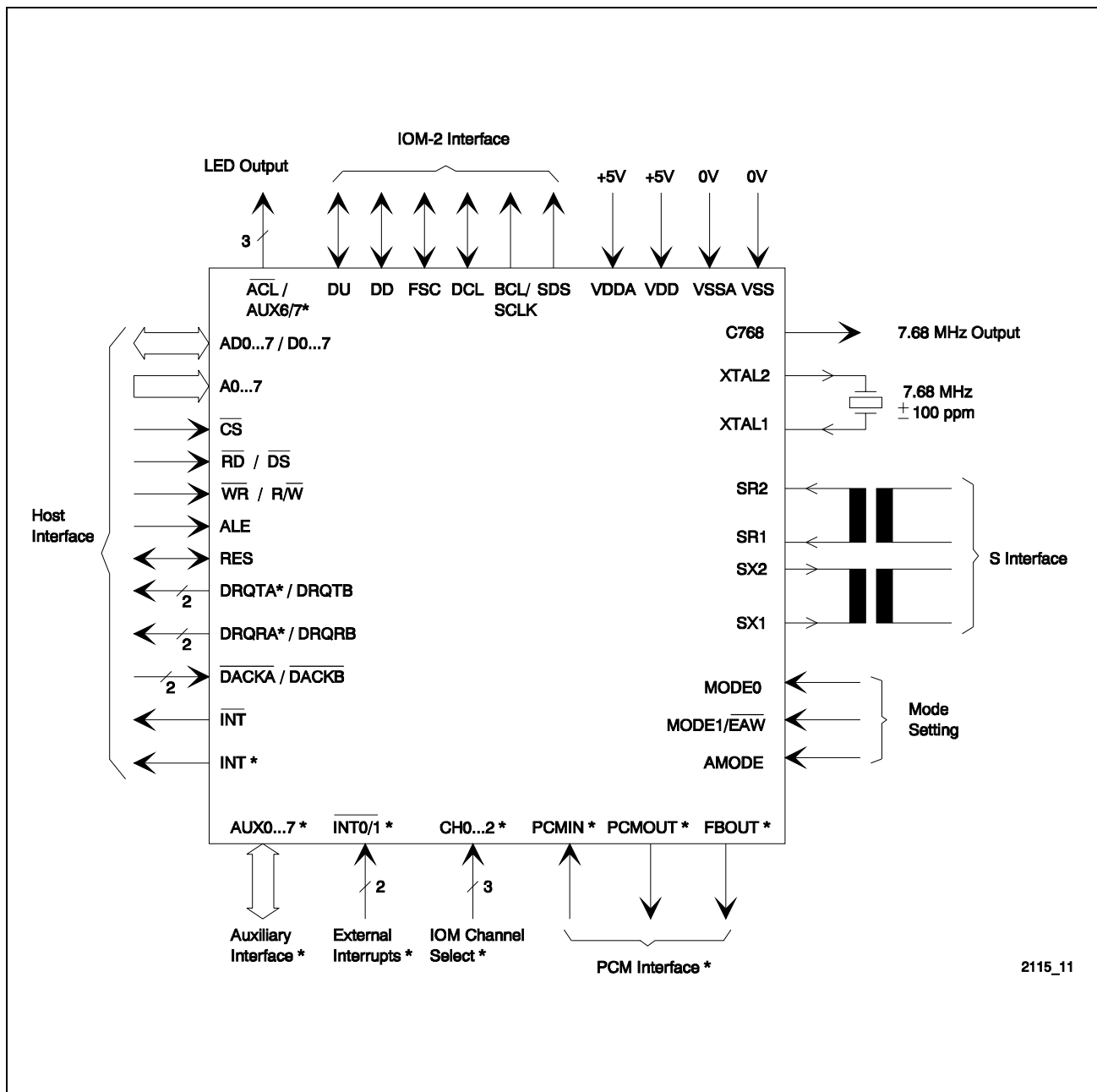
Figure 1 Logic Symbol
