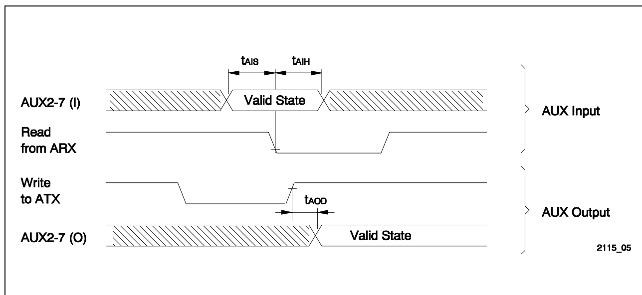
Figure 114 AUX Interface I/O Timing
