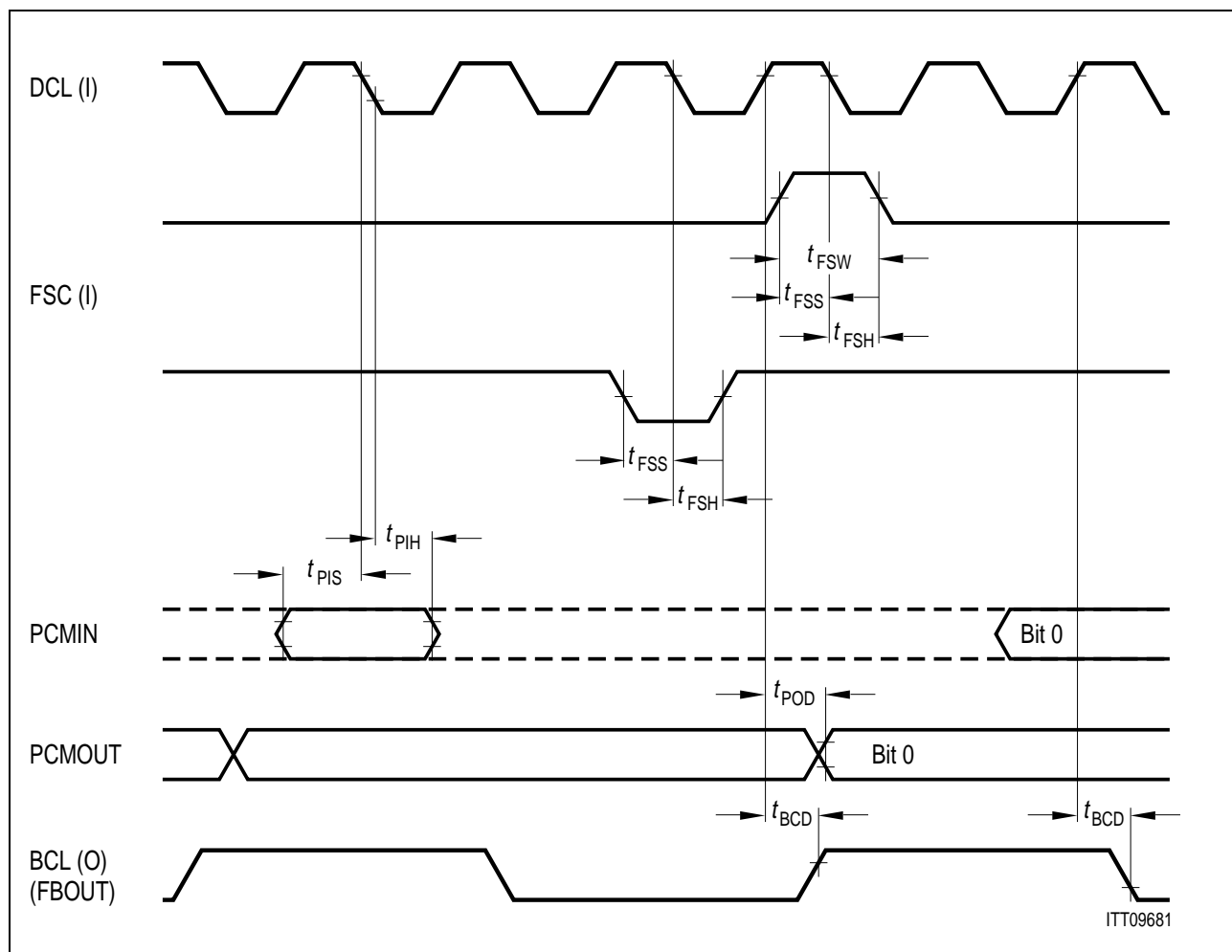
Figure 112 PCM Interface Timing (LT-S, LT-T mode)
