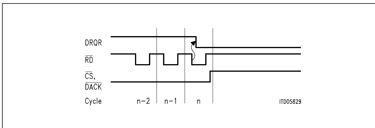
Figure 44 Timing Diagram for DMA-Transfers (slow or fast) Receive ( n = 4, 8, 16 \text{ or } 32 )
