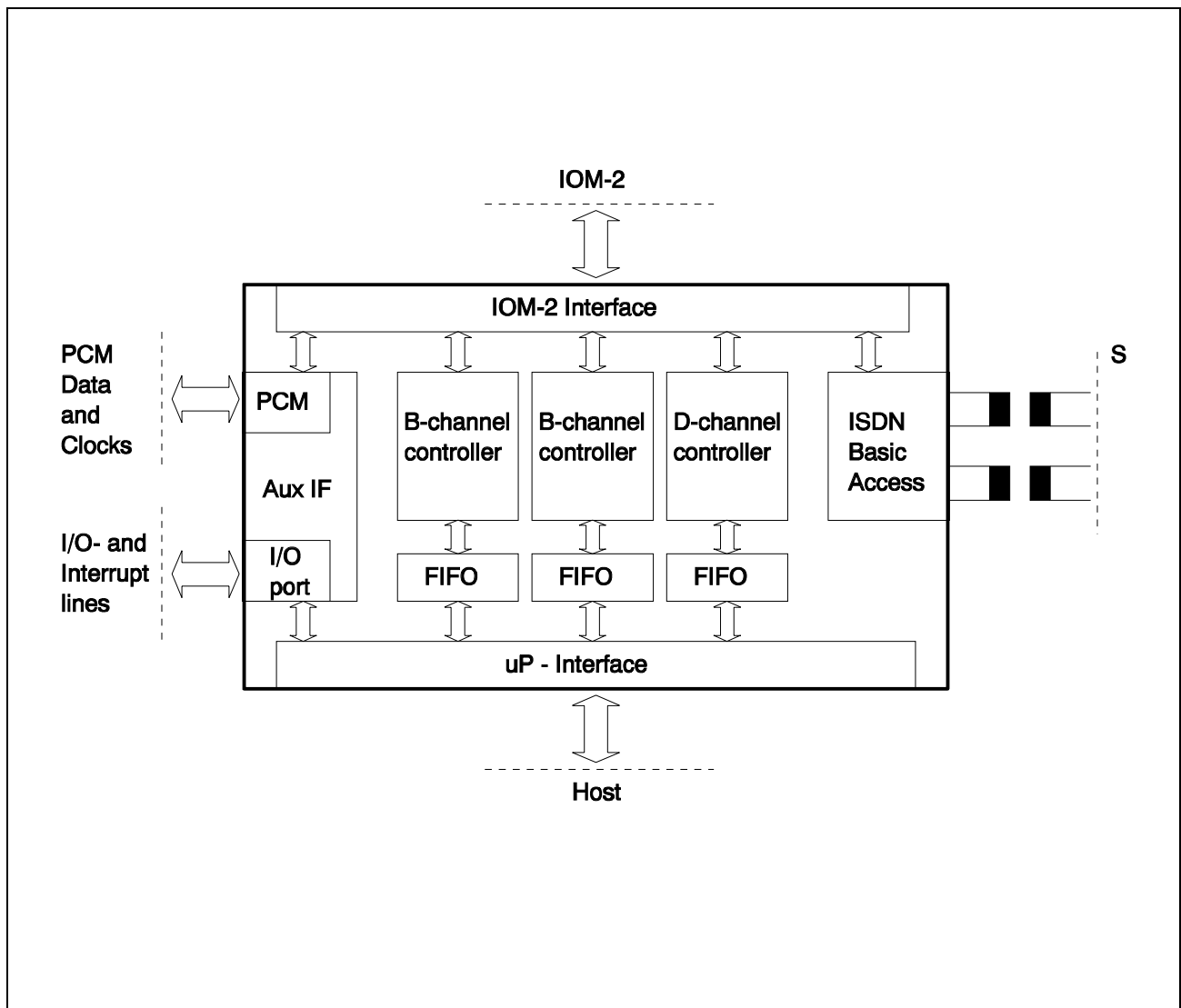
Figure 3 Block Diagram
