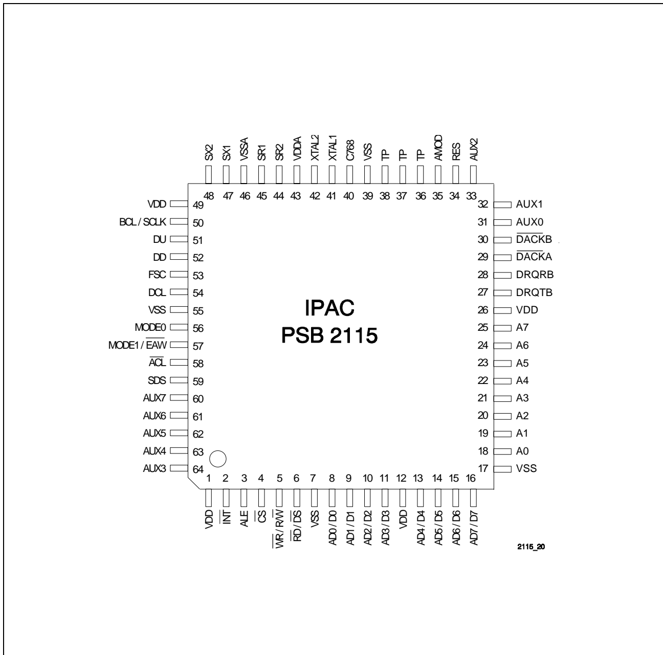
Figure 2 Pin Configuration
