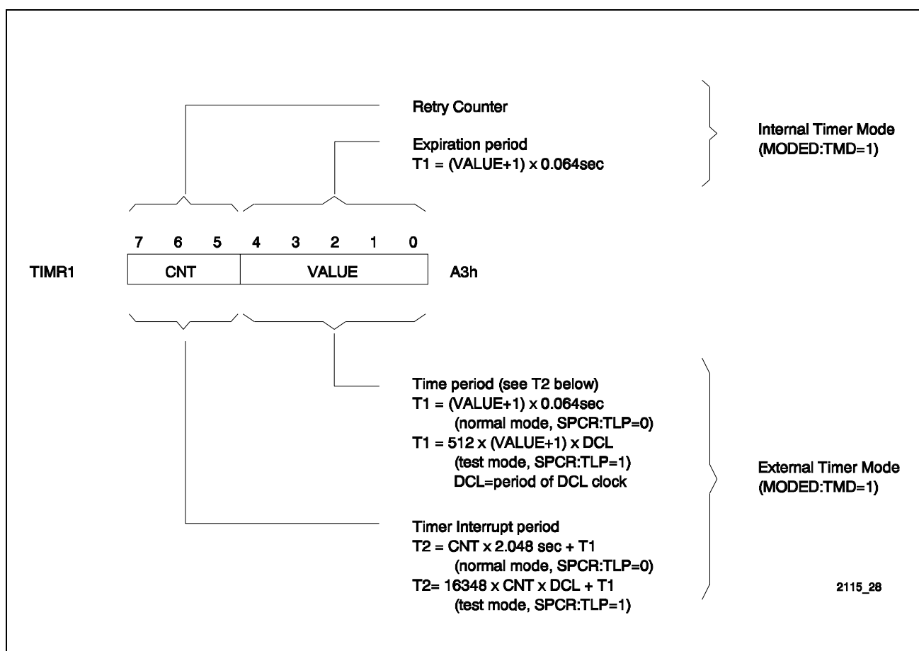
Figure 48 Timer 1 Register
