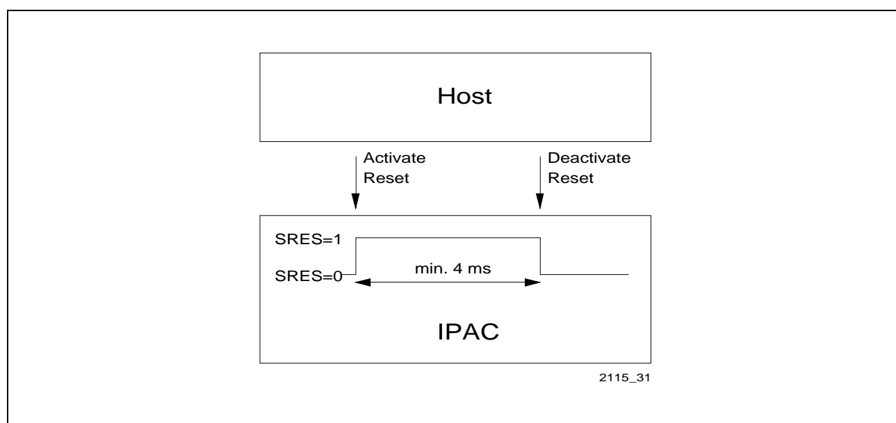
Figure 50 Reset Timing
