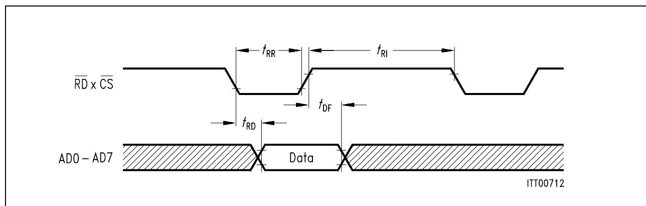
Figure 103 Microprocessor Read Cycle
