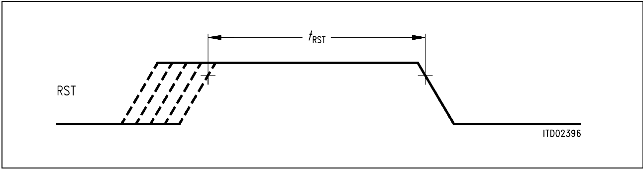
Figure 118 Reset Signal
