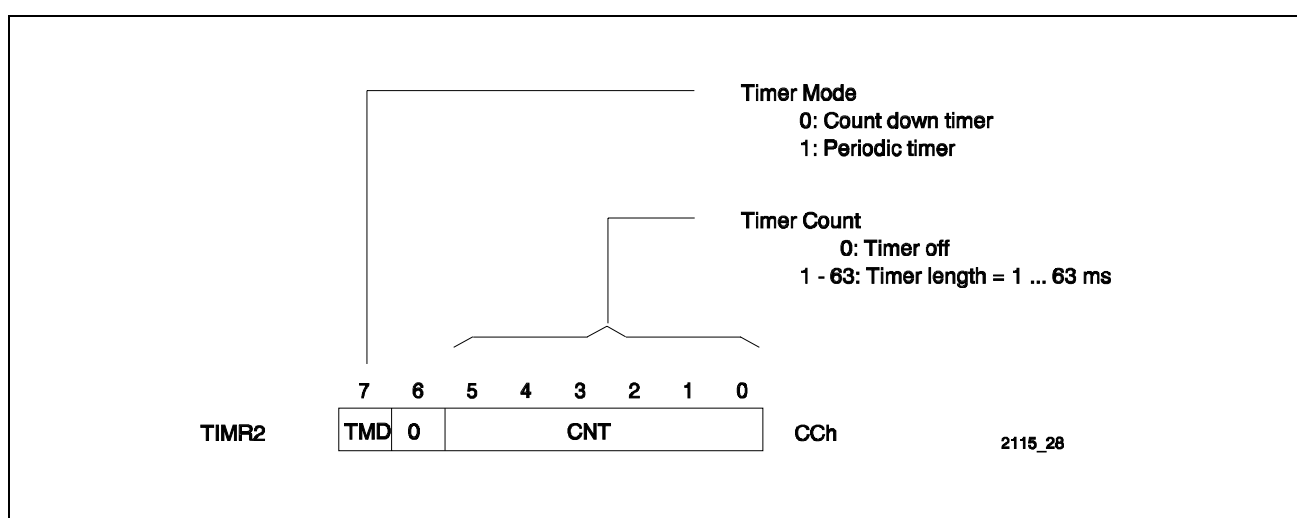
Figure 49 Timer 2 Register
