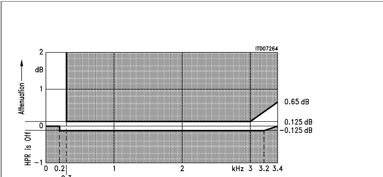
Figure 18 Receive: Reference Frequency 1014 Hz, Input Signal Level 0 dBm0
