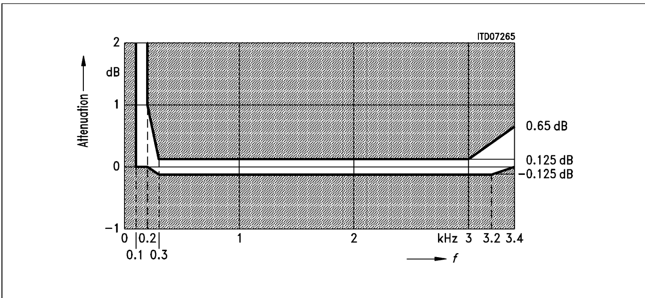
Figure 19 Transmit: Reference Frequency 1014 Hz, Input Signal Level 0 dBm0
