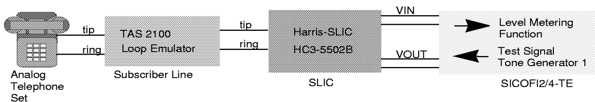
Figure 35 Test configuration
