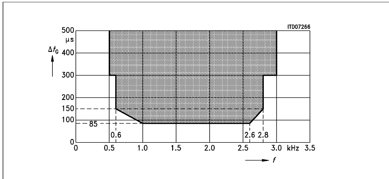
Figure 20 Group Delay Distortion Transmit: Input Signal Level 0 dBm0
