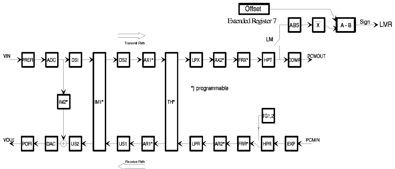
Figure 30 Block diagram of one SICOFI2/4-TE channel
