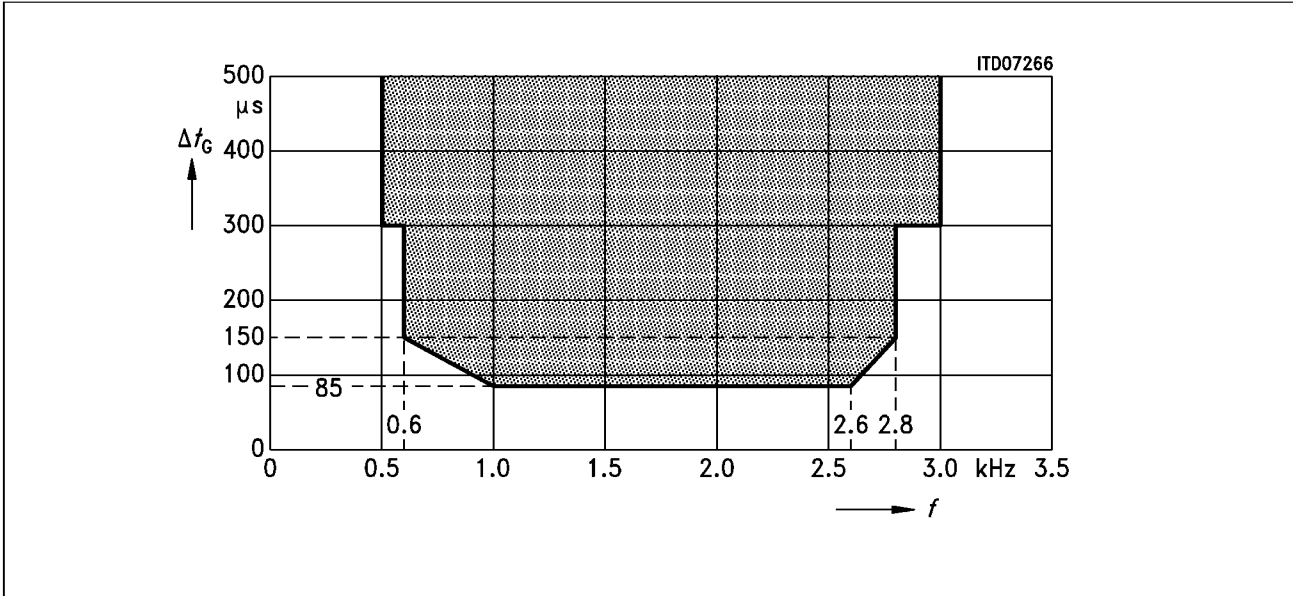
Figure 21 Group Delay Distortion Receive: Input Signal Level 0 dBm0 1)
