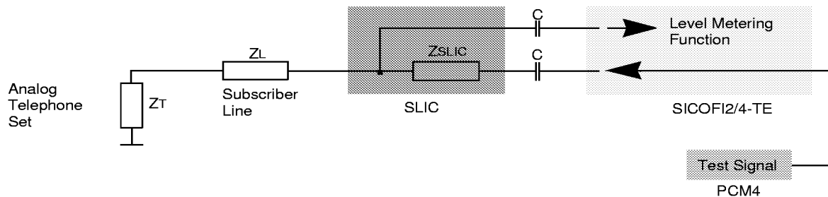
Figure 33 Test signal for level metering provided by PCM4
