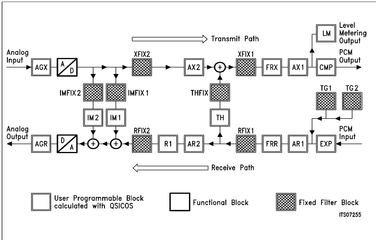
Figure 3 SICOFI®2/4-TE Signal Flow Graph (for any channel)
