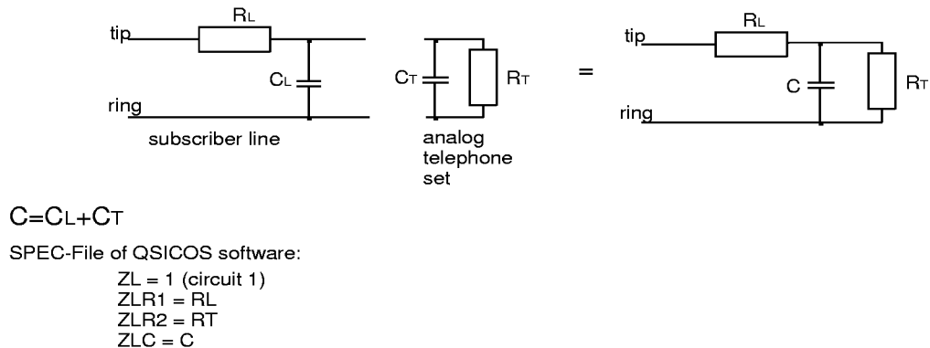
Figure 36 A simplified model of a subscriber line and an analog telephone set
