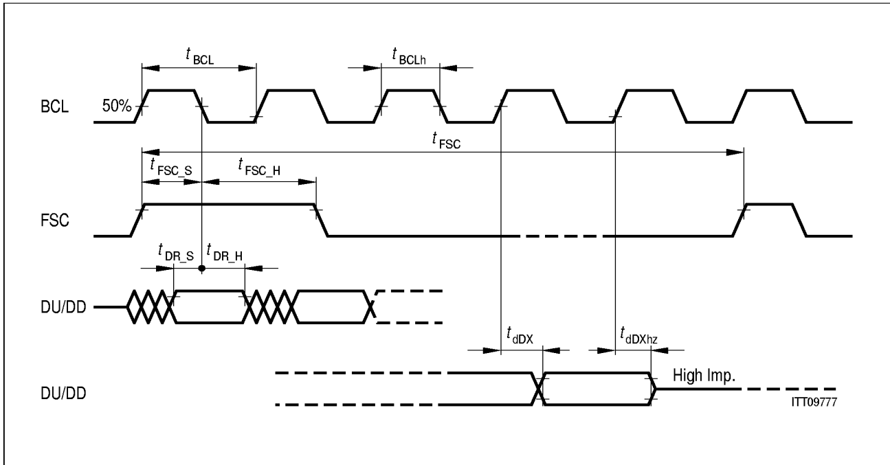
Figure 38 Single Clocking Mode
