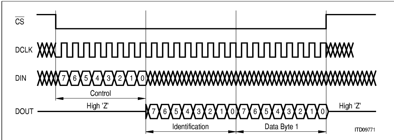
Figure 7 Example for a Read Access, with One Data Byte Transferred via DOUT
