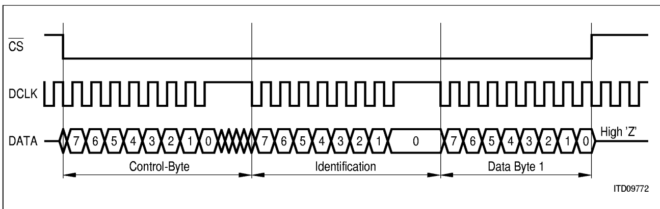
Figure 8 Example for a Write/Read Access, with a Byte by Byte Transfer, and DIN and DOUT Strapped Together
