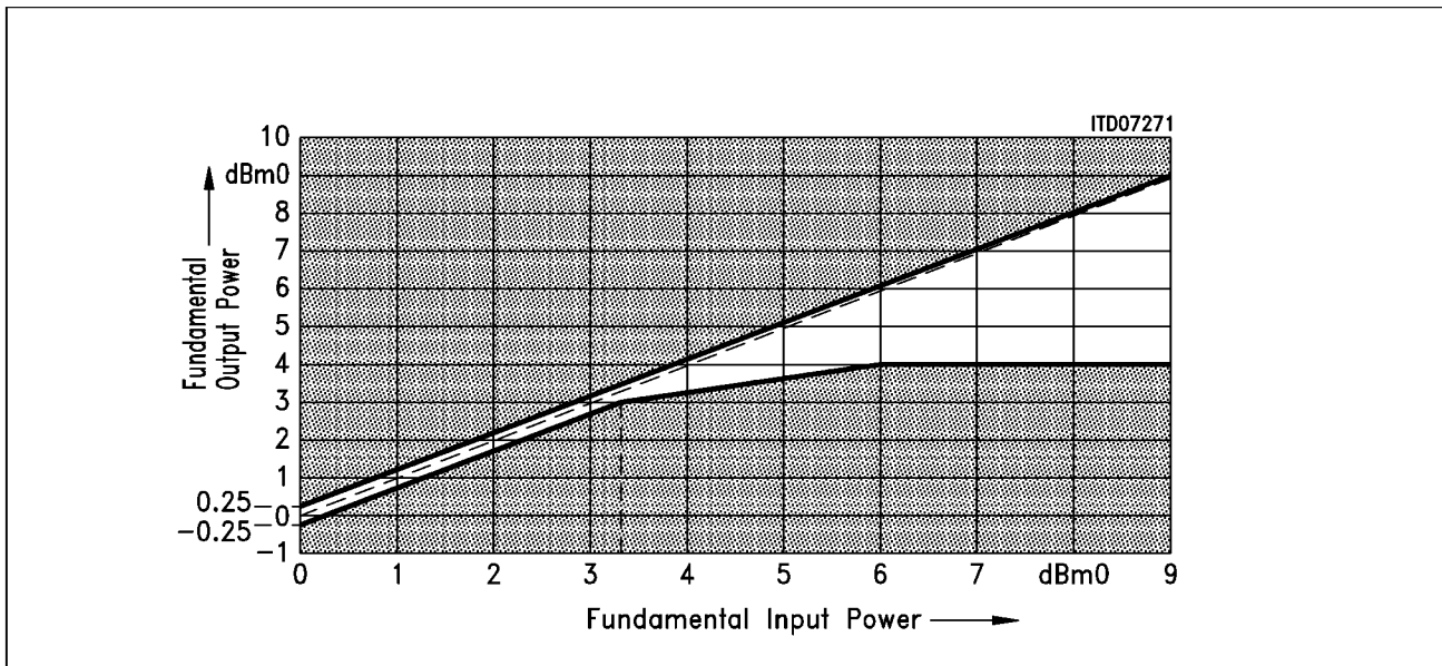
Figure 25 \mu -Law, Transmit: measured with sine wave f = 1014 Hz.
