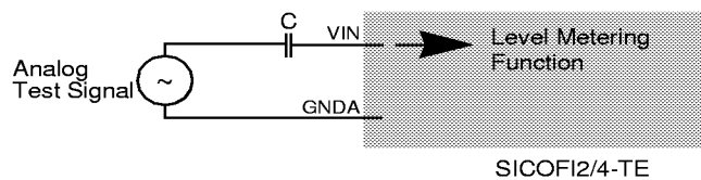
Figure 34 Measurement of an unknown level
