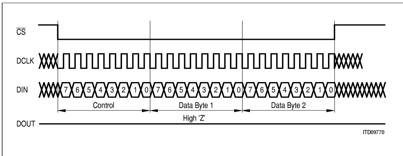
Figure 6 Example for a Write Access, with Two Data Bytes Transferred
