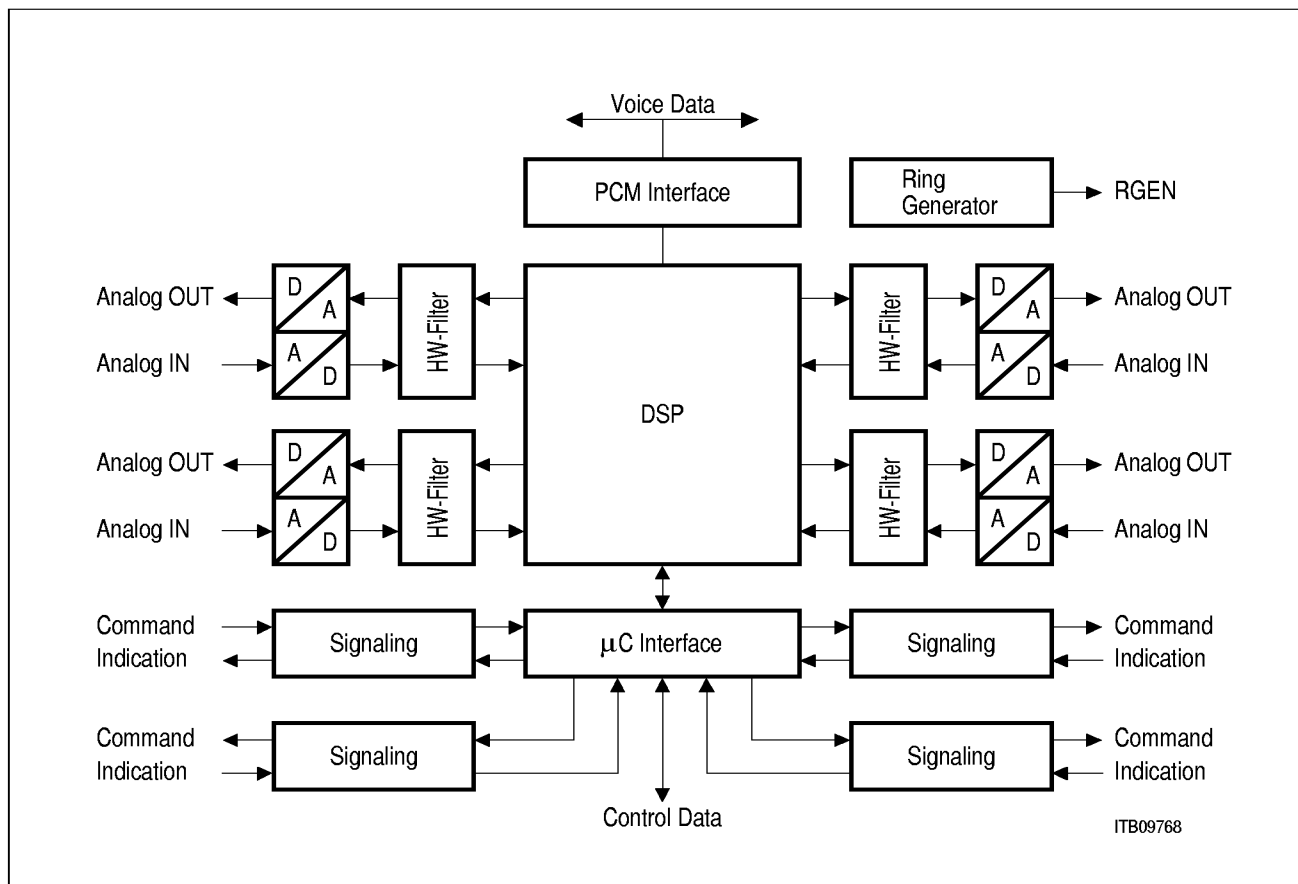
Figure 4 SICOFI2/4®-TE Block Diagram
