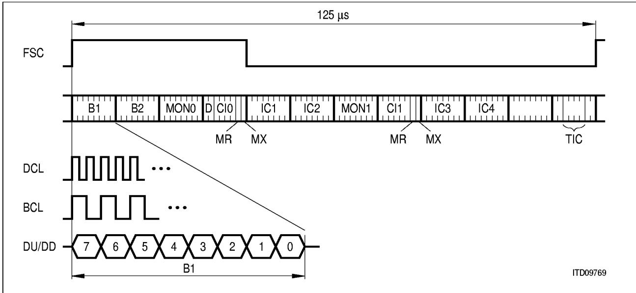
Figure 5 Example for IOM-2 Terminal Mode
