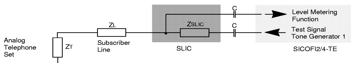
Figure 32 Test signal generated by tone generator 1
