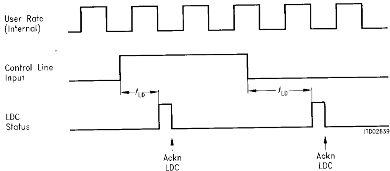
Figure 58 Asynchronous DCE Interface
