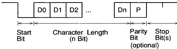
Figure 30 Asynchronous Character Format
