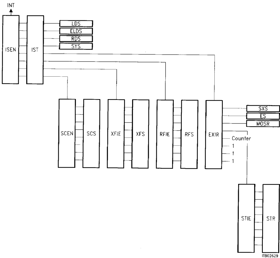
Figure 44 Interrupt Structure
