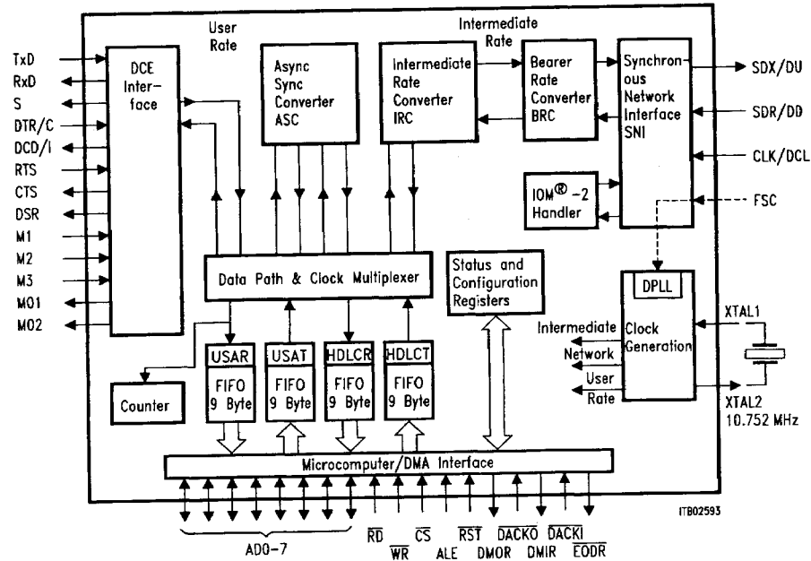
Figure 1 Block Diagram
