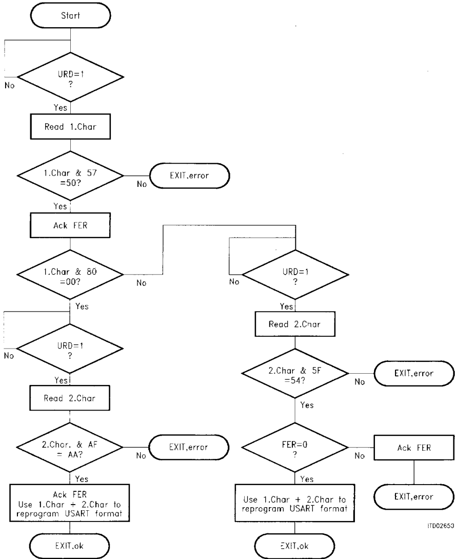
Figure 72 Flow Diagram
