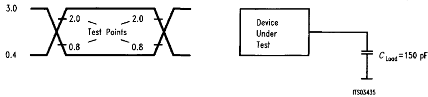
Figure 49 Input/Output Waveform for AC Tests
