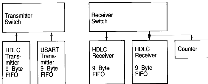
Figure 28 Serial Communication Logic
