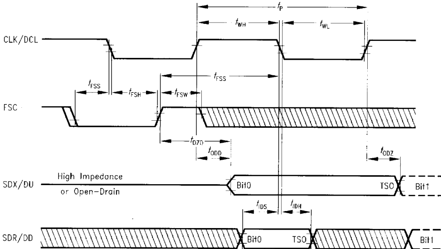
Figure 55 PCM Interface Timing
