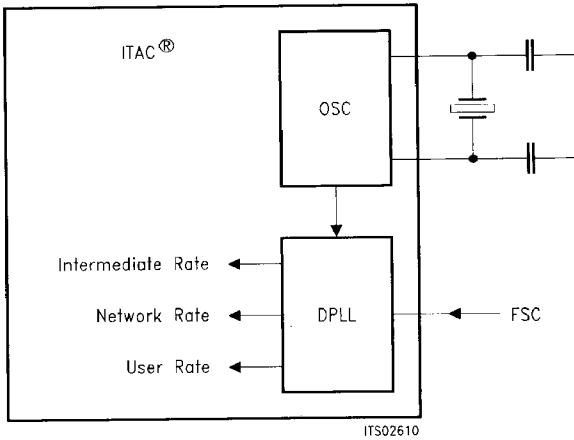
Figure 18 Clock Synchronization
