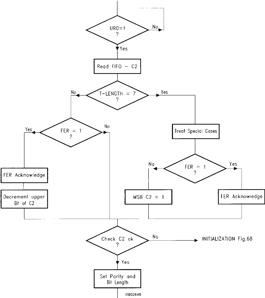
Figure 70 Reception of Character of T/t (C2)
