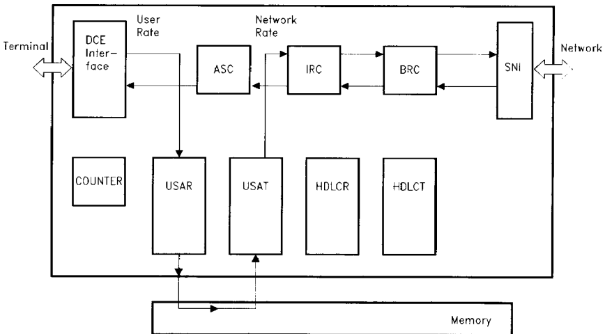
Figure 3 Terminal Adapter for Unequal Speeds
