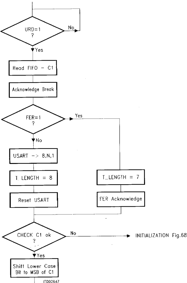
Figure 69 Reception of Remaining Bits of A/a (C1)
