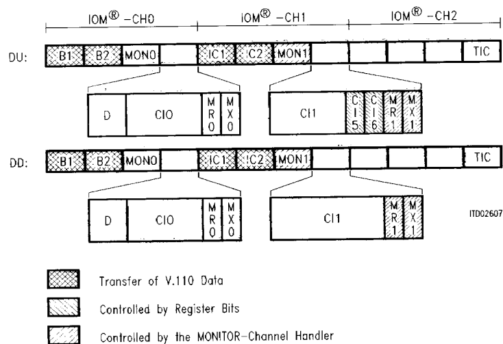
Figure 15 IOM ® -2 Interface Support
