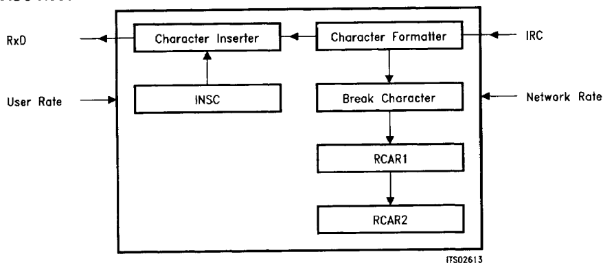
Figure 21 ASC Receiver
