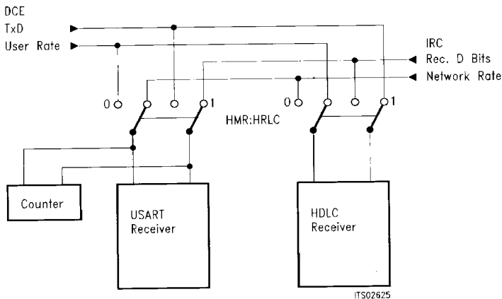
Figure 40 Data Path for the Receiver Blocks
