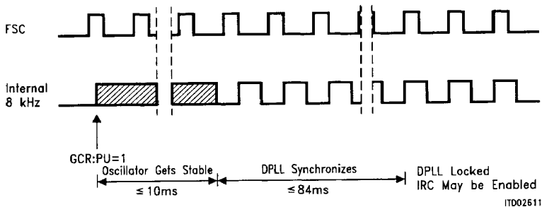
Figure 19 Synchronization of the DPLL
