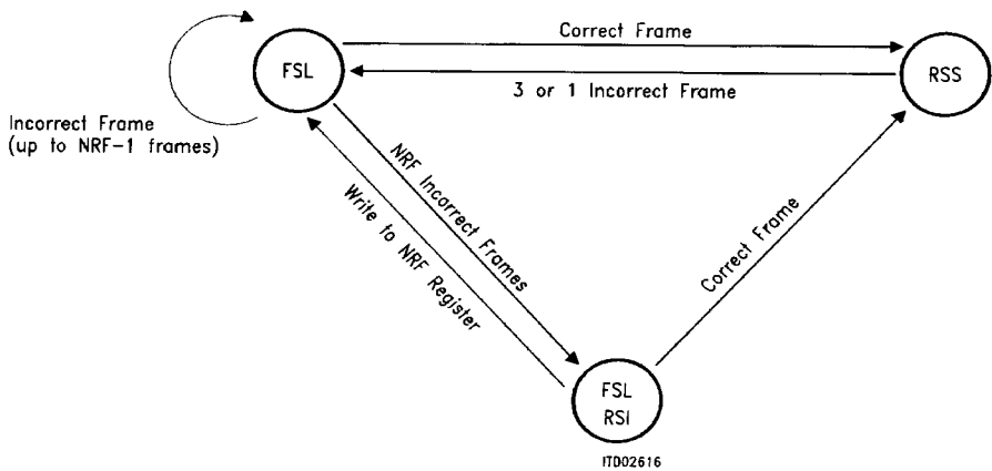
Figure 26 Synchronization State Machine
