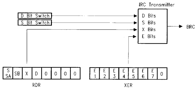
Figure 24 IRC Transmitter
