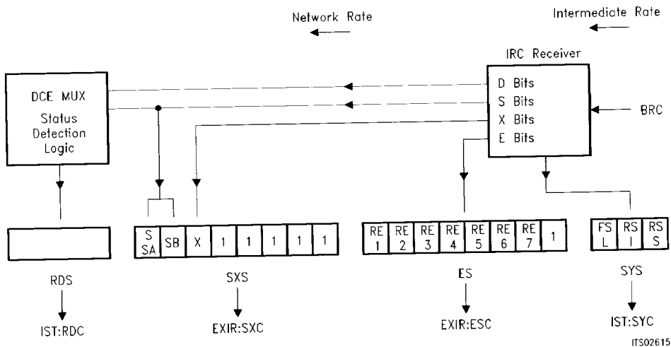
Figure 25 IRC Receiver
