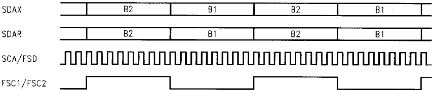
Figure 60 Signals of the SSI Interface
