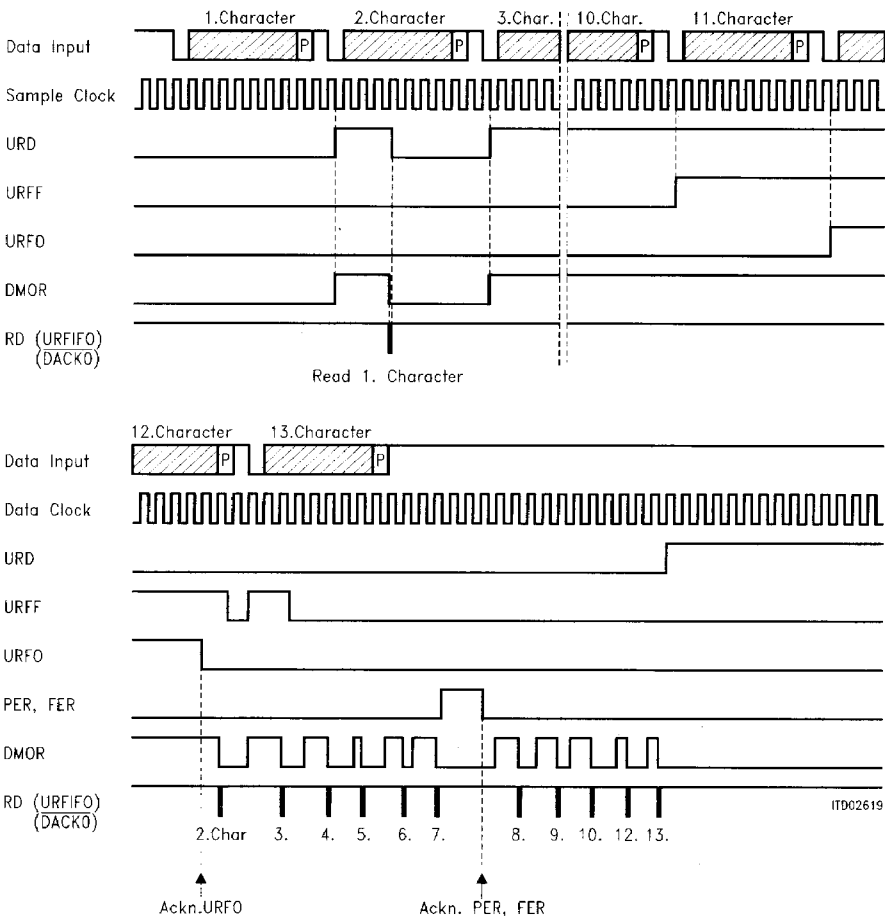
Figure 32 URFIFO Handling
