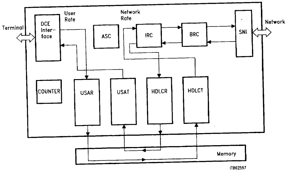
Figure 5 Terminal Adapter for V.120 or DMI
