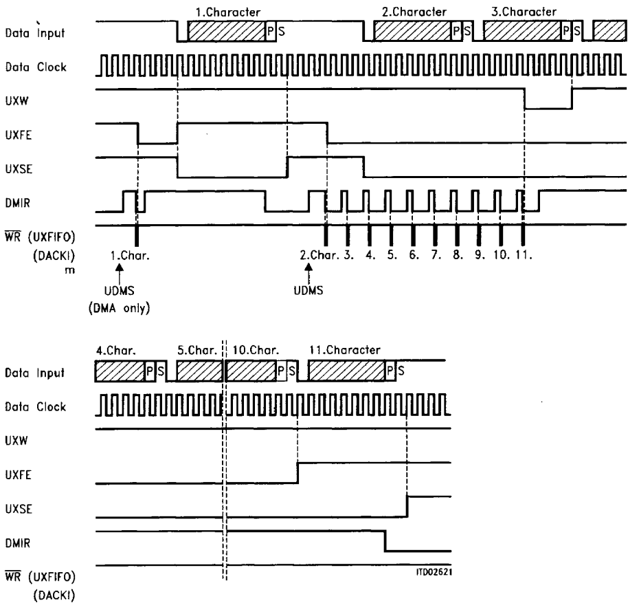
Figure 34 UXFIFO Handling
