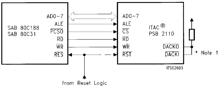
Figure 11 Connecting the ITAC ® to SAB 80C188/80C31
