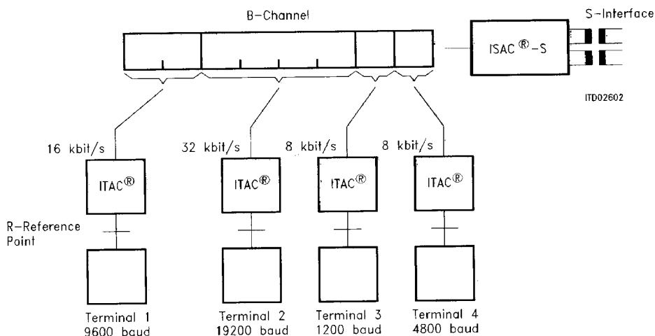
Figure 10 Sharing of Bearer Channel Among Several Independent DTEs
