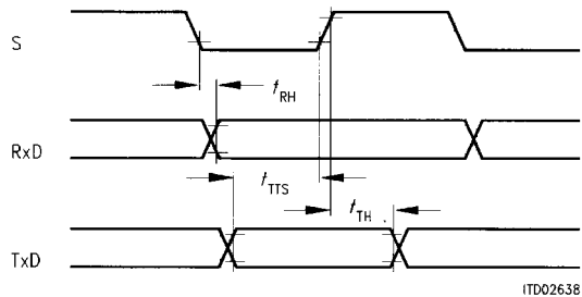
Figure 57 Synchronous DCE Interface Timing
