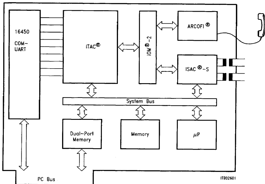
Figure 9 Add-On Cards for PCs
