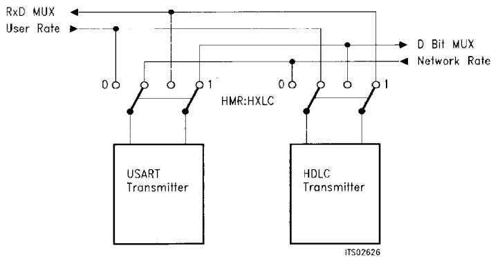
Figure 41 Data Path for the Transmitter Blocks
