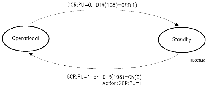
Figure 47 Standby State Diagram (GCR:V24 = 1)
