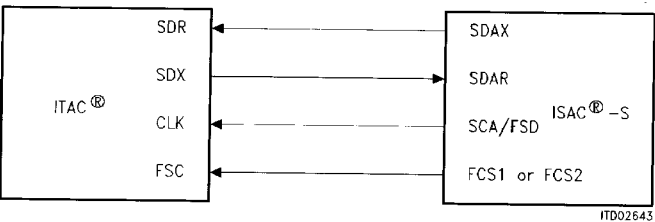
Figure 62 Connecting the ITAC ® and the ISAC ® -S via SSI
