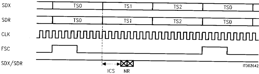
Figure 61 Signals of the Serial Network Interface (time-slot 1, ICS = 3, NR = 9600 bit/s)
