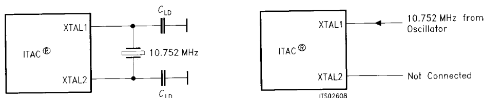
Figure 16 Connection of Clock Sources
