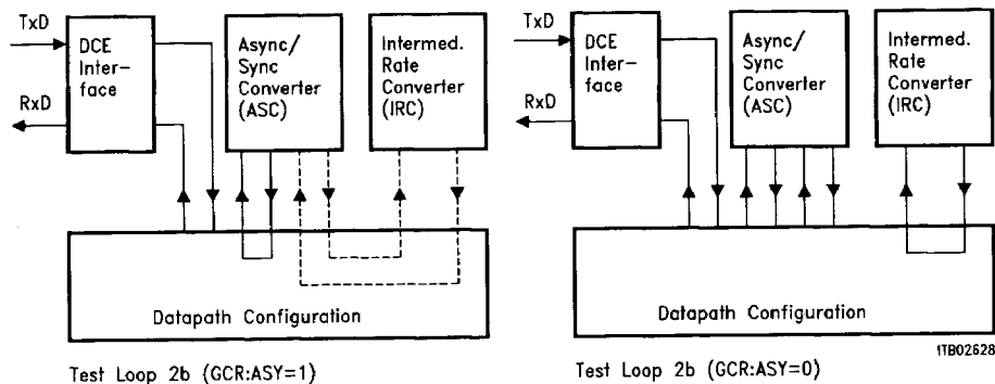
Figure 43 Test Loop 2b
