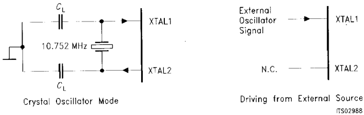
Figure 48 Oscillator Circuits
