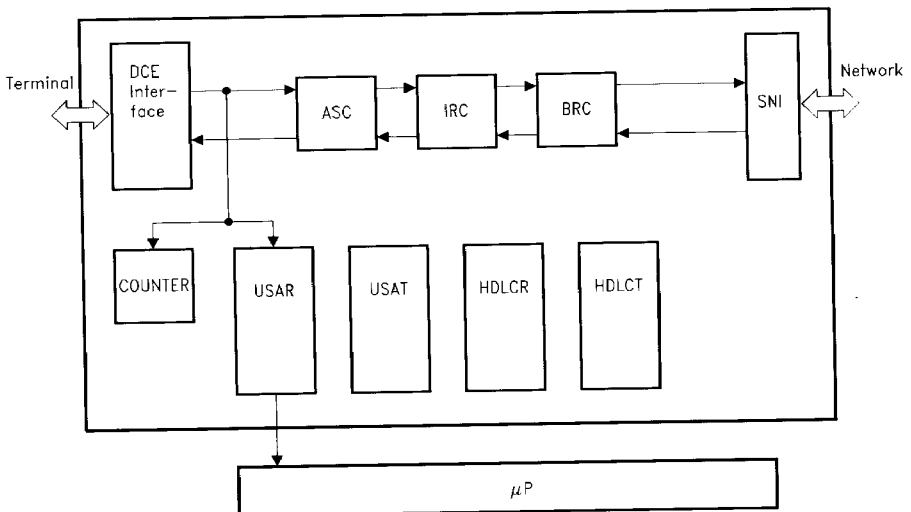
Figure 2 Transparent Mode. User Rate = Network Rate
