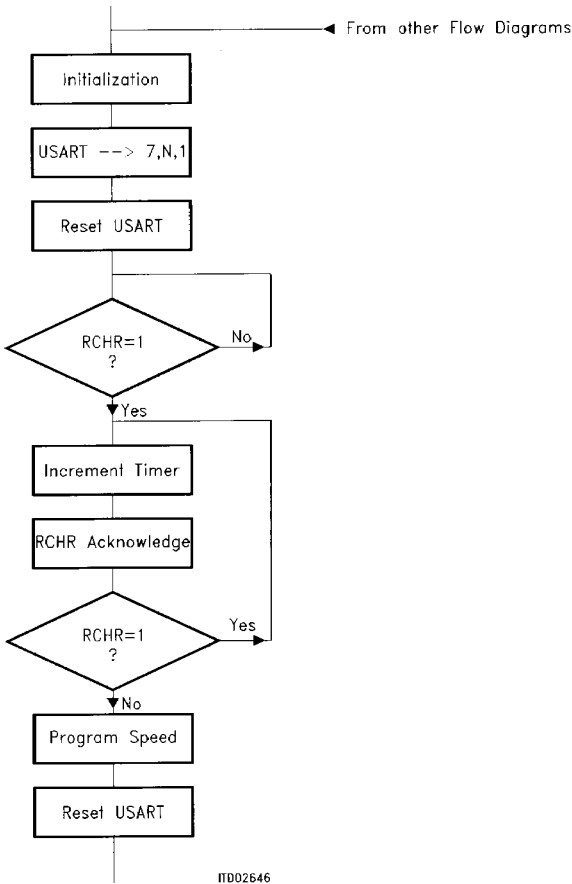
Figure 68 Speed Recognition Flow Diagram
