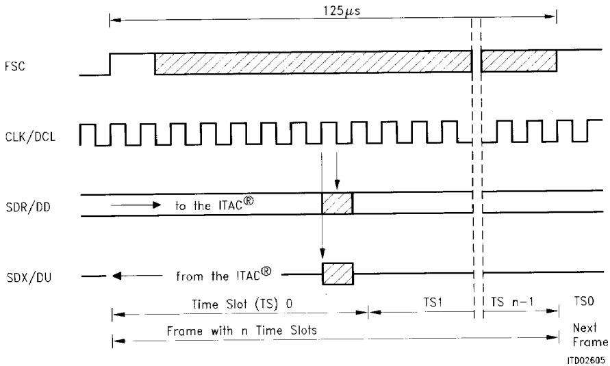
Figure 13 PCM Interface (single bit clock)
