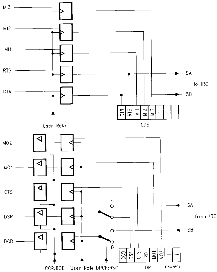
Figure 12 DCE Interchange Circuits (GCR:V24 = 1)
