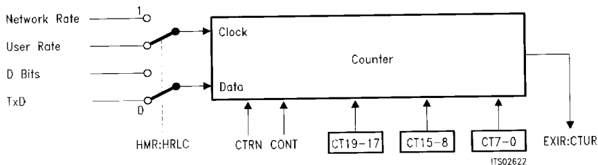
Figure 35 Counter
