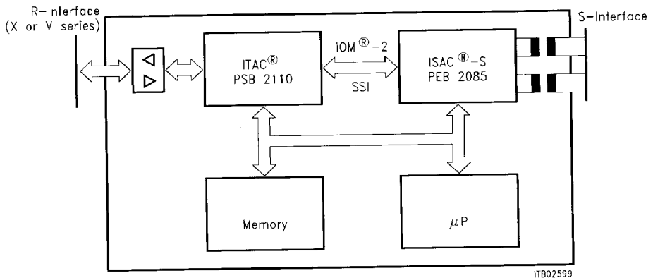
Figure 7 Terminal Adapter for ISDN Basic Access
