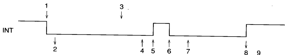
Figure 46 Service Program for Edge -Triggered Interrupt Controllers
