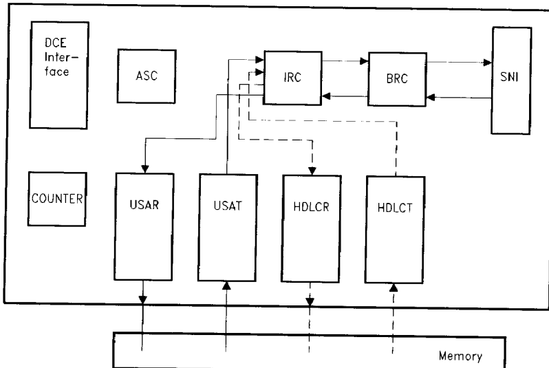
Figure 6 Data Transfer from or to the Local Memory
