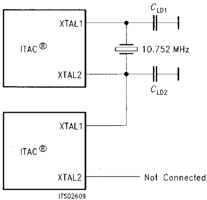
Figure 17 Driving Two ITAC® Oscillators by One Crystal
