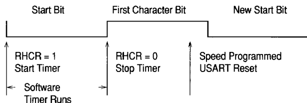
Figure 64 Speed Measurement
