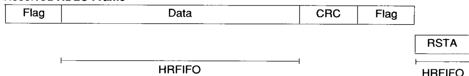
Figure 36 Received HDLC Frame
