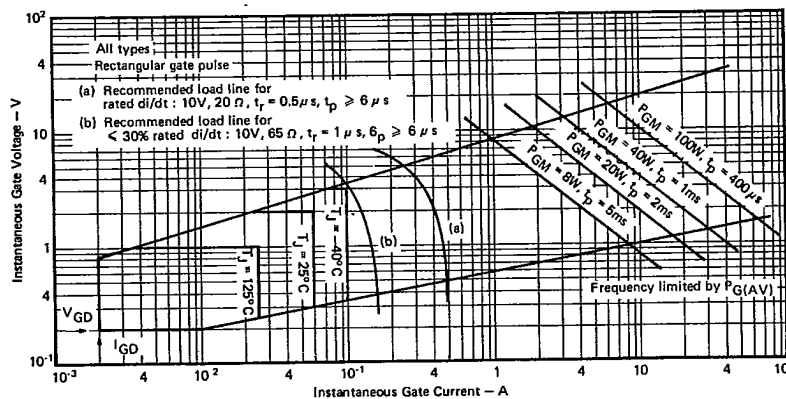
Fig. 9 - Gate Characteristics / Fig. 10 - Area of All Possible Triggering Points
