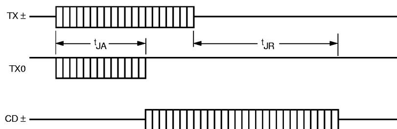
Figure 8. Jabber Timing
