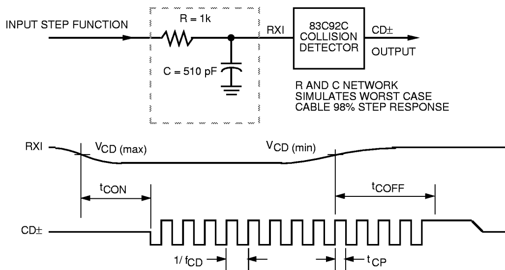
Figure 6. Collision Timing
