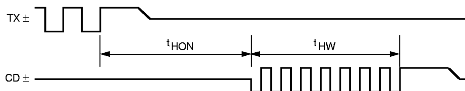
Figure 7. Heartbeat Timing
