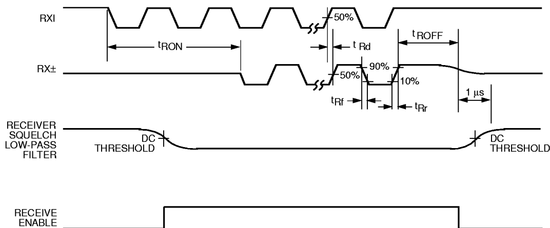
Figure 4. Receiver Timing
