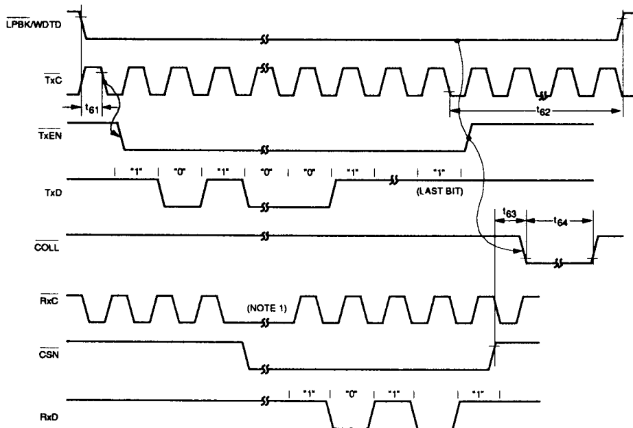
Figure 14. Loopback Timing — (Cont.)
