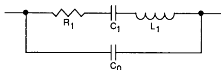
EQUIVALENT CIRCUIT OF CRYSTAL
