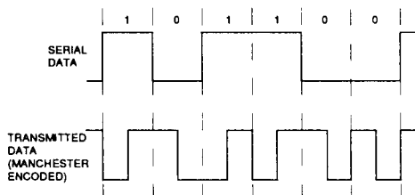
Figure 2. Manchester Coding
