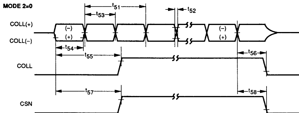
Figure 11. Collision Timing
