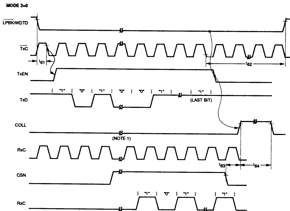
Figure 13. Loopback Timing
