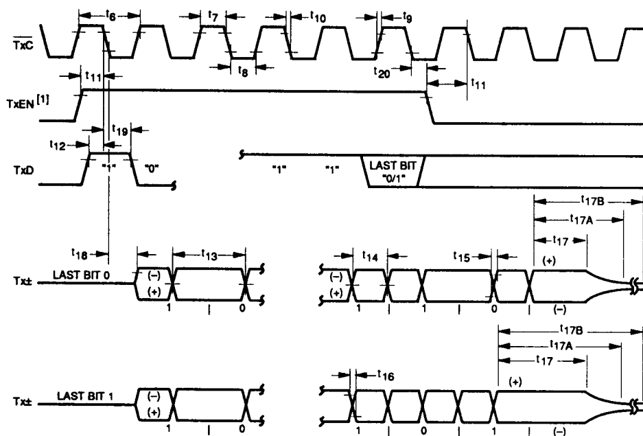
Figure 7. Transmit Timing
