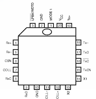
PLASTIC LEADED CHIP CARRIER TOP VIEW
