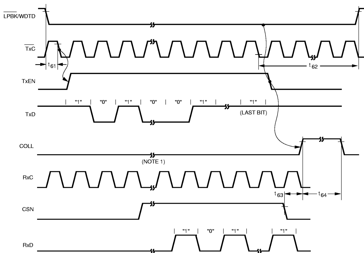
Figure 13. Loopback Timing
