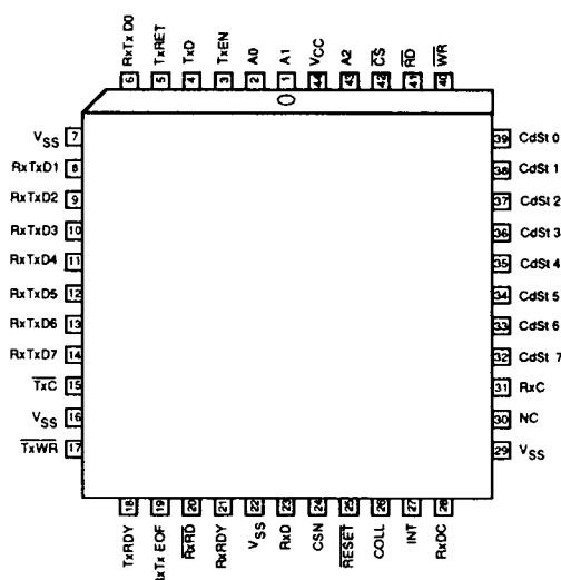
Figure 2. Plastic Leaded Chip Carrier Top view
