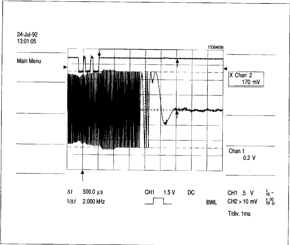
Figure 12 Lock-In Time for GSM Application
