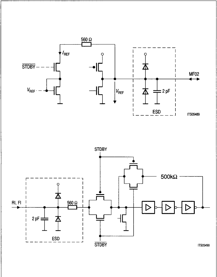
Figure 5 Equivalent I/O Schematics (cont'd)
