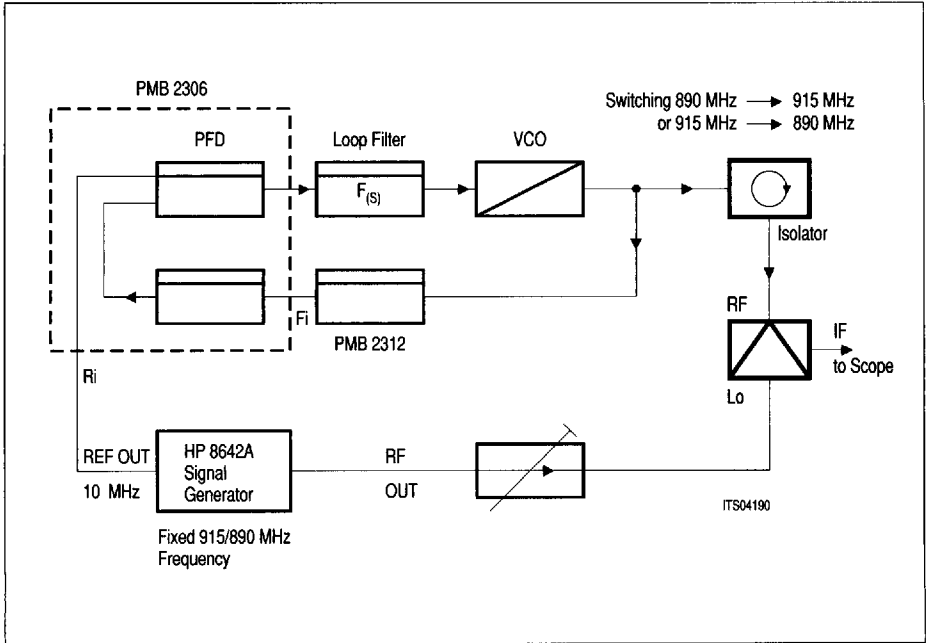
Figure 13 Measurement Set-Up for Lock-In Time
