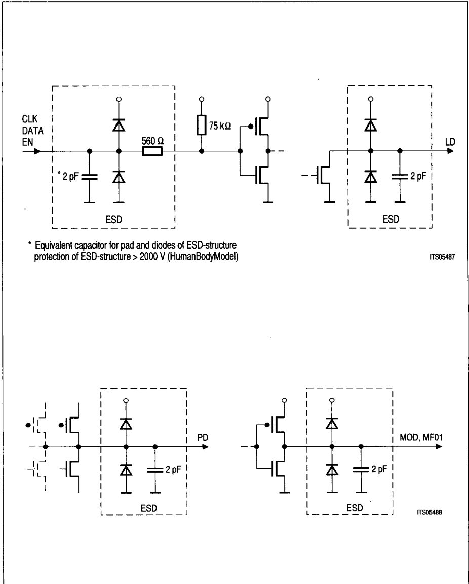
Figure 4 Equivalent I/O Schematics
