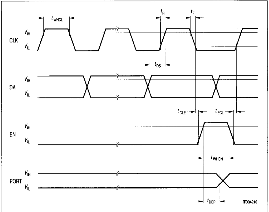
Figure 7 Serial Control Data Input Timing
