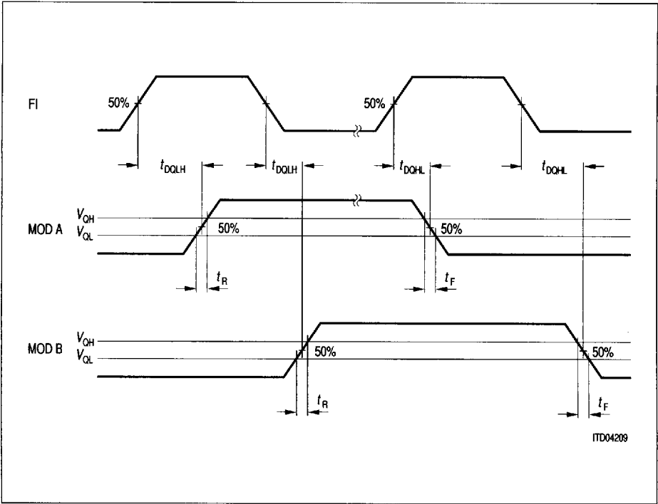
Figure 6 Modulus Control Output Timing
