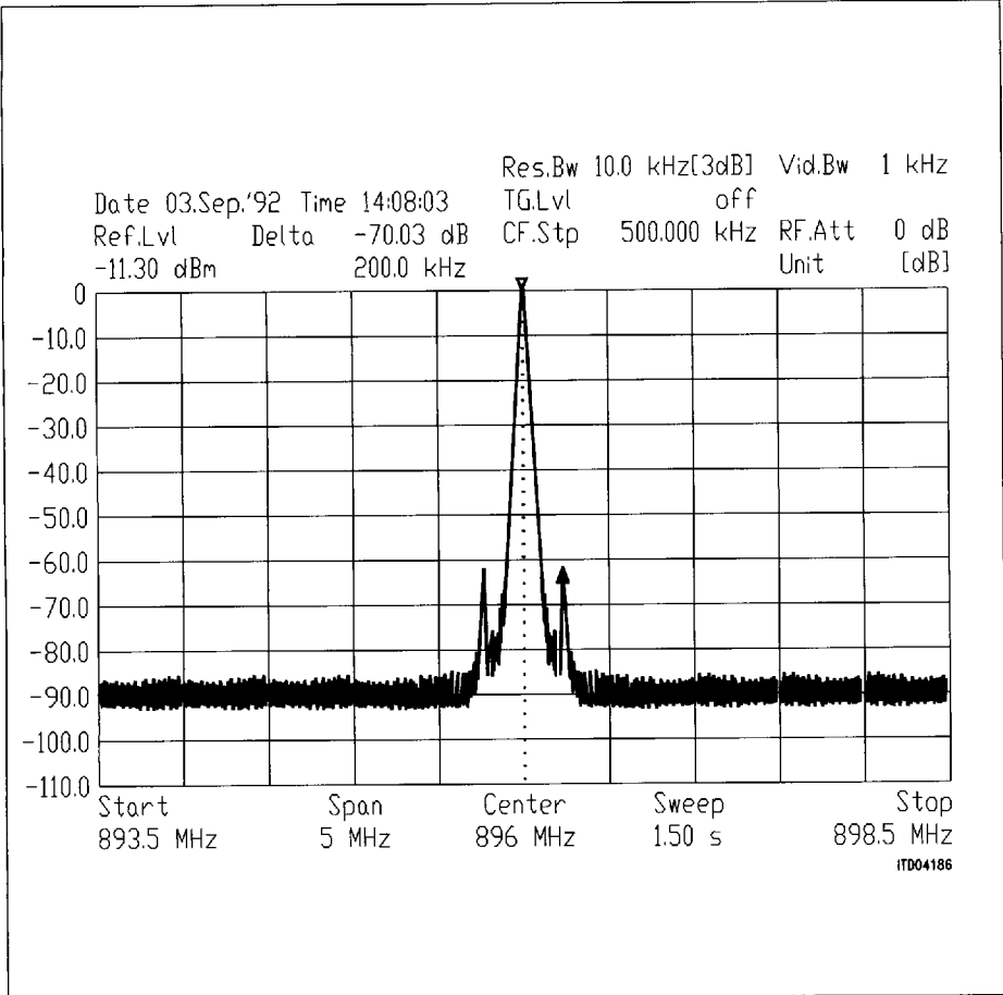
Figure 11 Spectrum at Lower End of GSM TX Board (Mobile)
