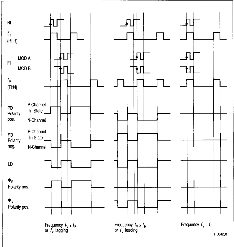
Figure 3 Phase Detector Output Waveforms
