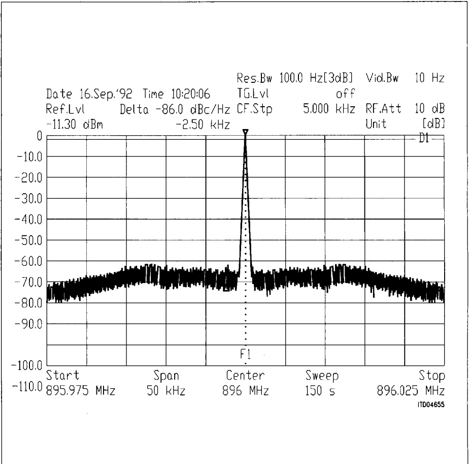
Figure 10 Phase Noise Close to the Carrier
