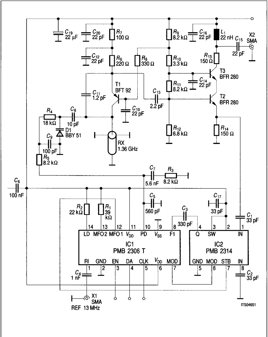
Figure 9 GSM Application Circuit
