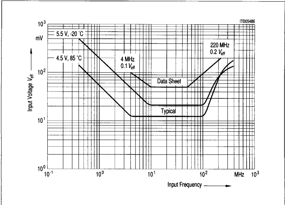
Figure 8 Input Sensitivity Signal FI (single HF-mode)
