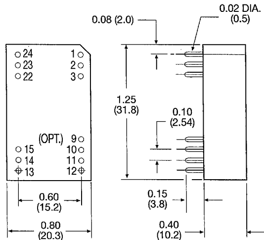
ALL DIMENSIONS INCHES (mm)
