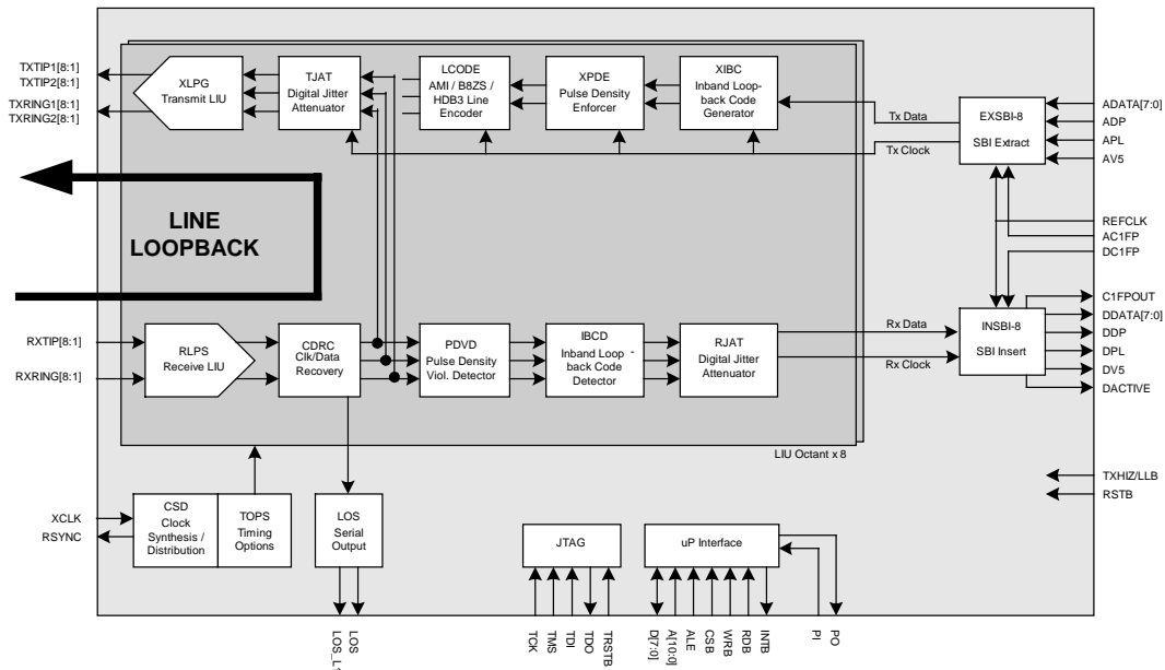
Figure 13 Line Loopback
