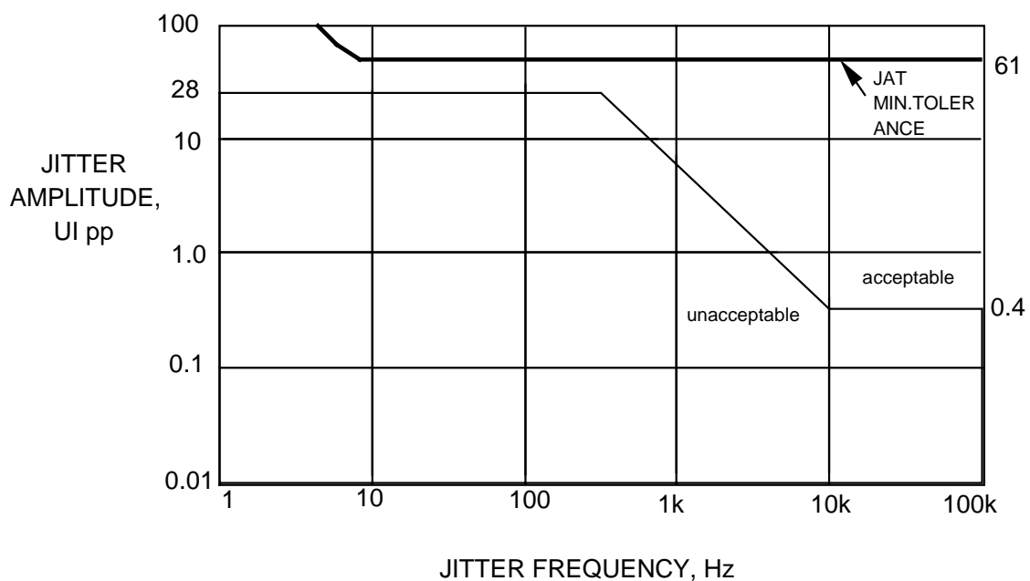
Figure 8 TJAT Jitter Tolerance
