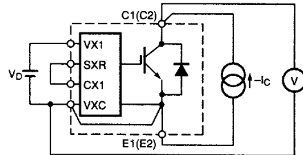
Figure 2 V_{EC} Test
