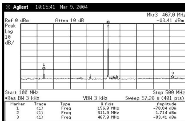
Figure 4: Spectrum Analysis at 311.04 MHz Analog Frequency Multiplier (2x) with sub-harmonics below -72 dBc
