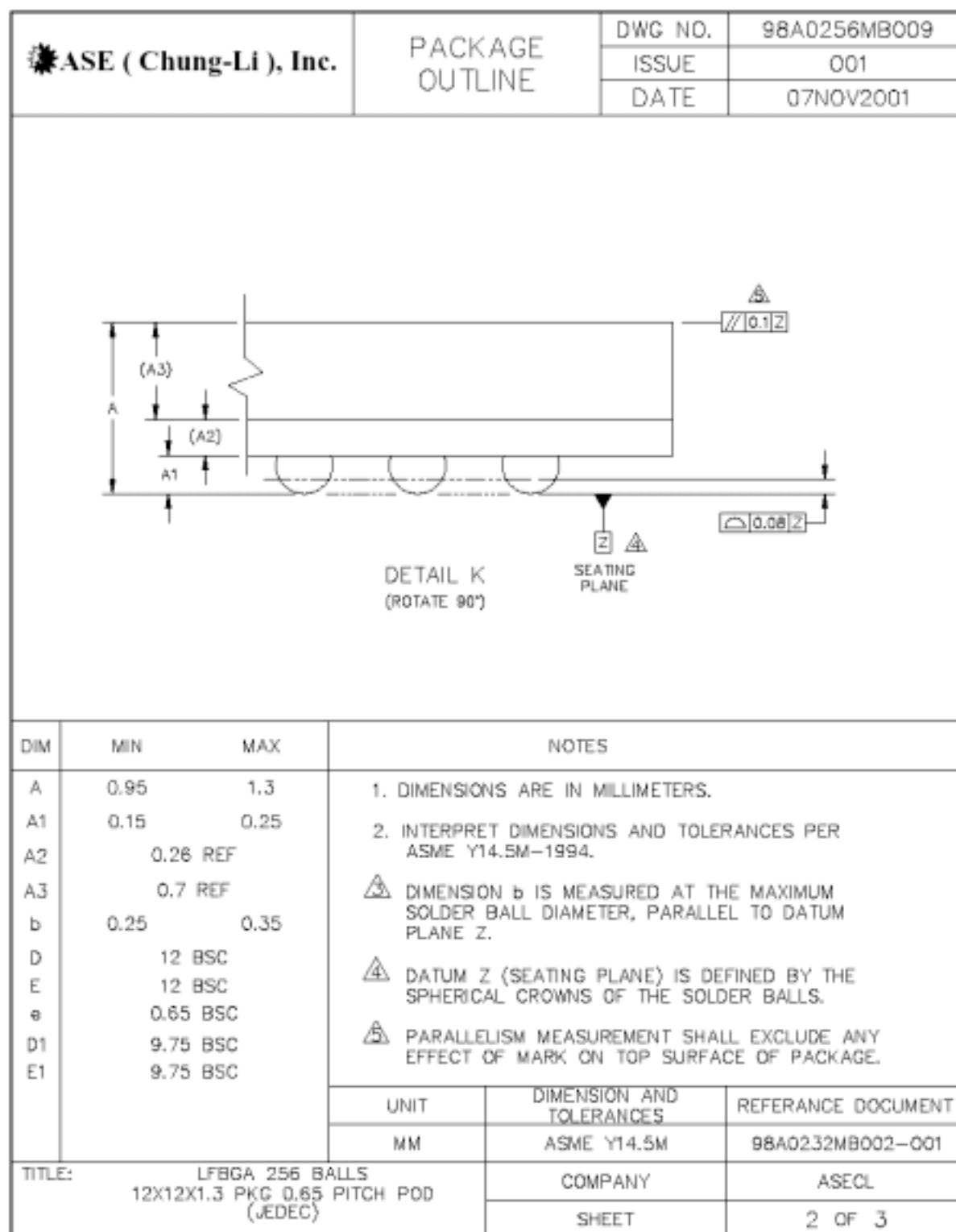
Figure 5-1b Package Dimension Diagram of PL-2519
