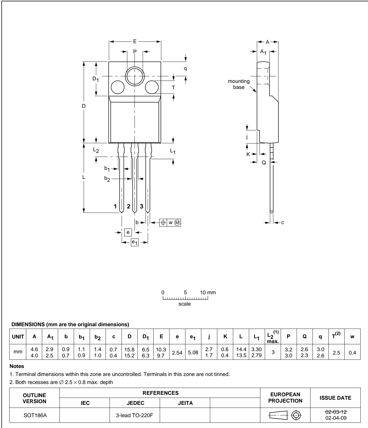
Fig 14. SOT186A (TO-220F).
