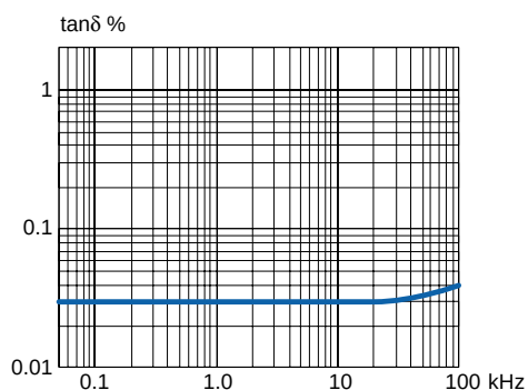
Dissipation factor vs. frequency (at +23 ^{\circ}\text{C} )
