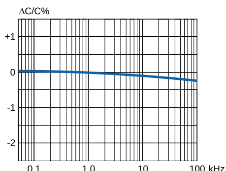
Capacitance vs. frequency (at +23 ^{\circ}\text{C} )
