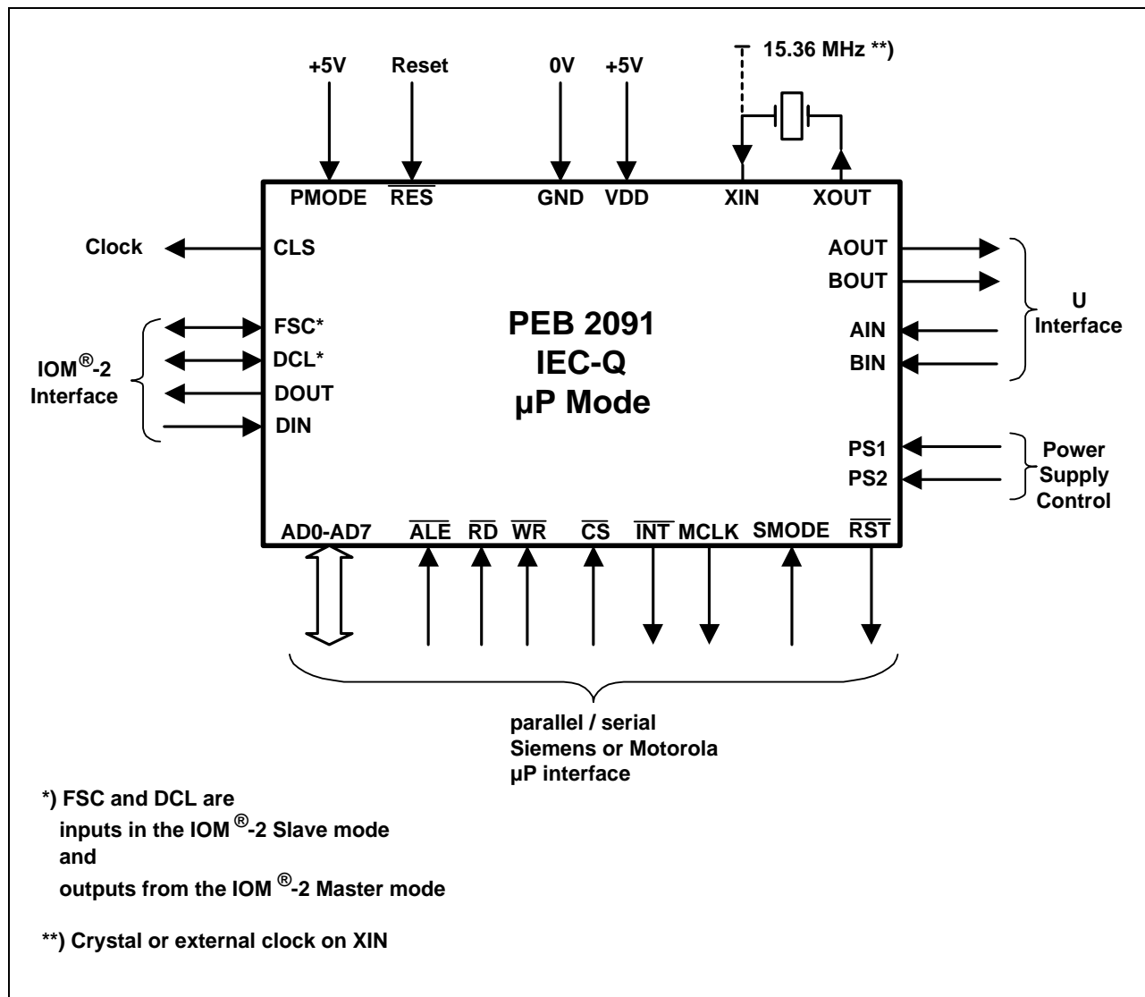
Figure 1 Logic Symbol for \mu P Mode
