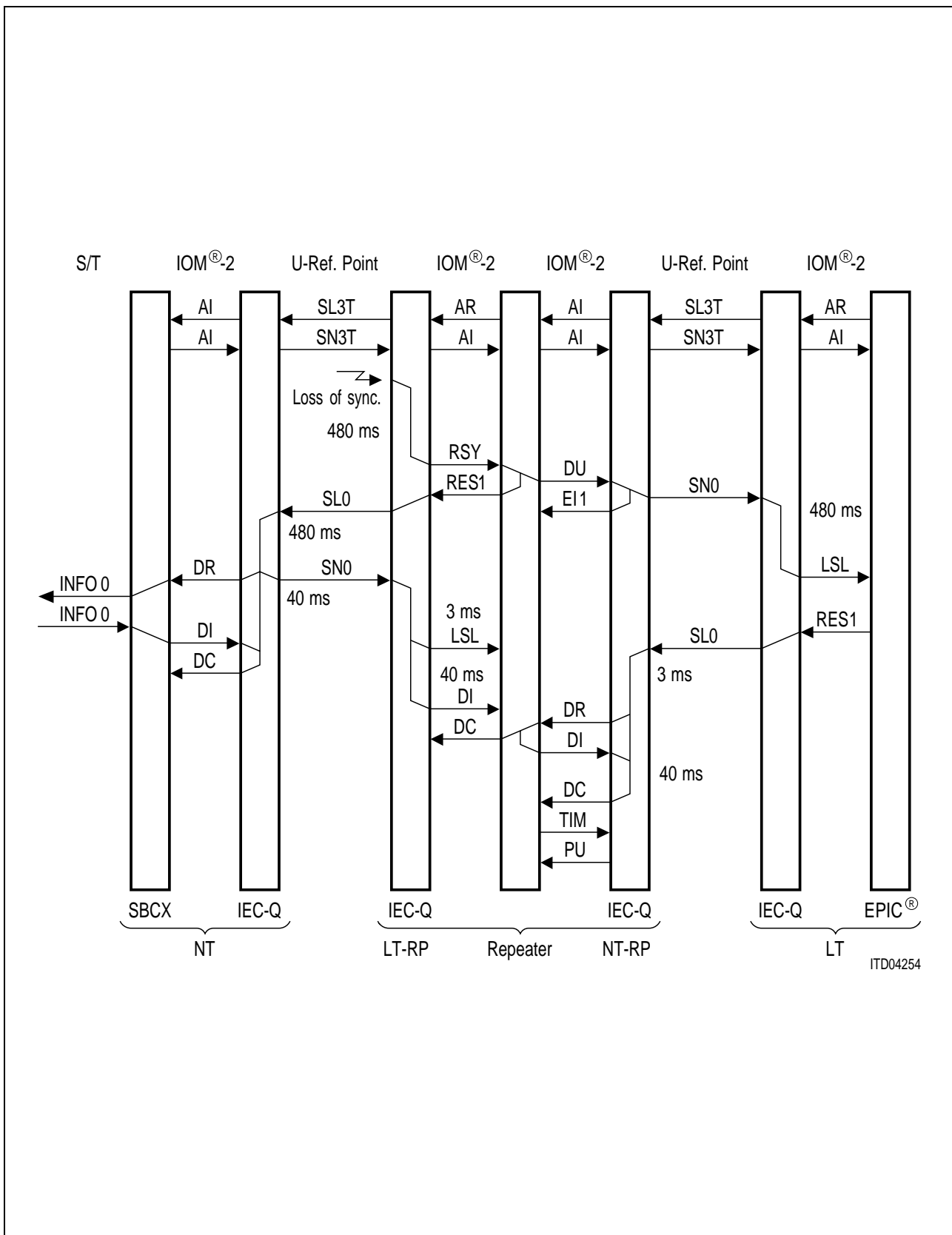
Figure 66 Loss of Synchronization at Repeater (NT side)
