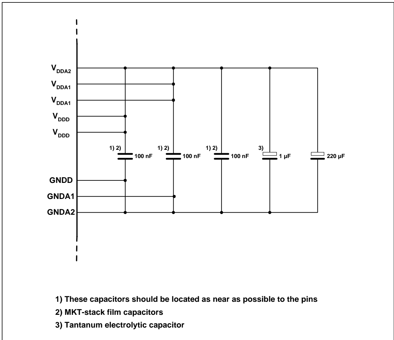
Figure 92 Power Supply Blocking
