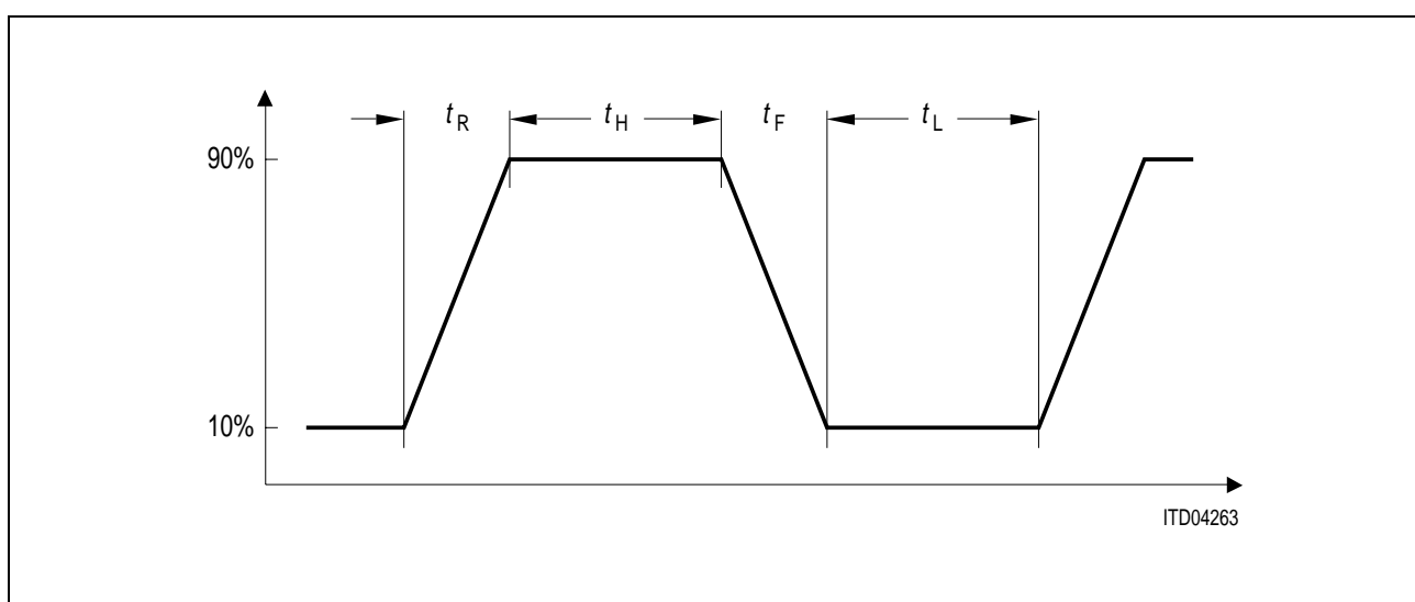
Figure 120 Dynamic Characteristics of the Duty Cycle
