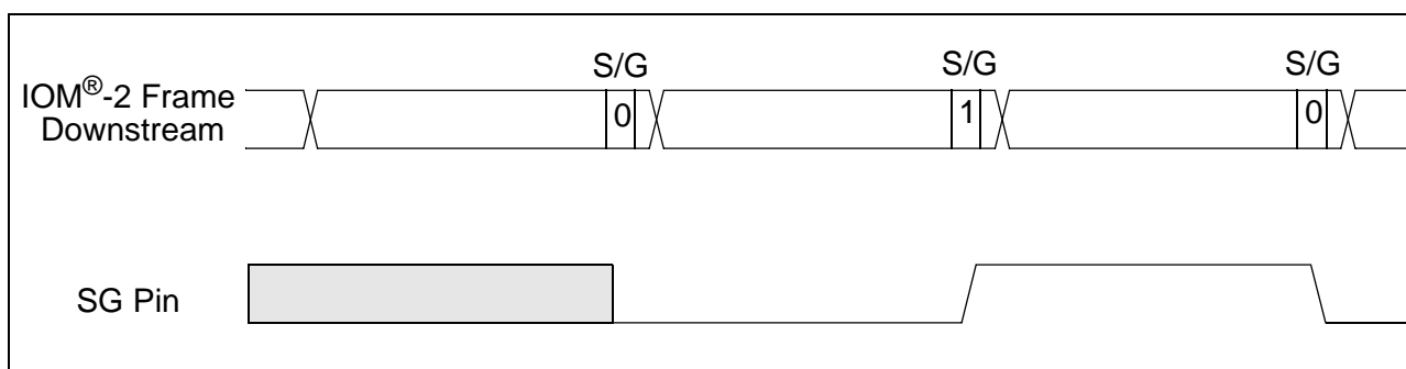
Figure 89 S/G Bit Status on Pin SG
