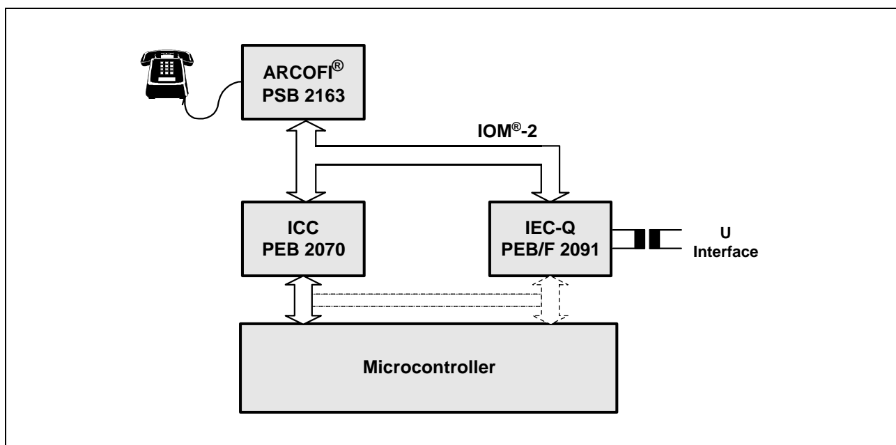
Figure 8 TE Application
