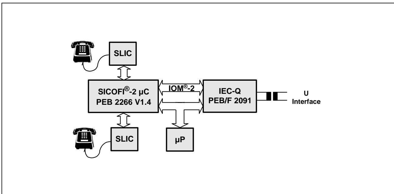
Figure 4 RT Application
