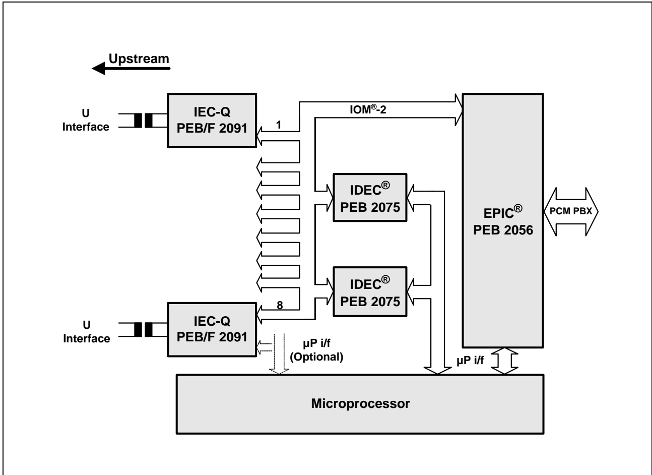
Figure 10 NT-PBX Application
