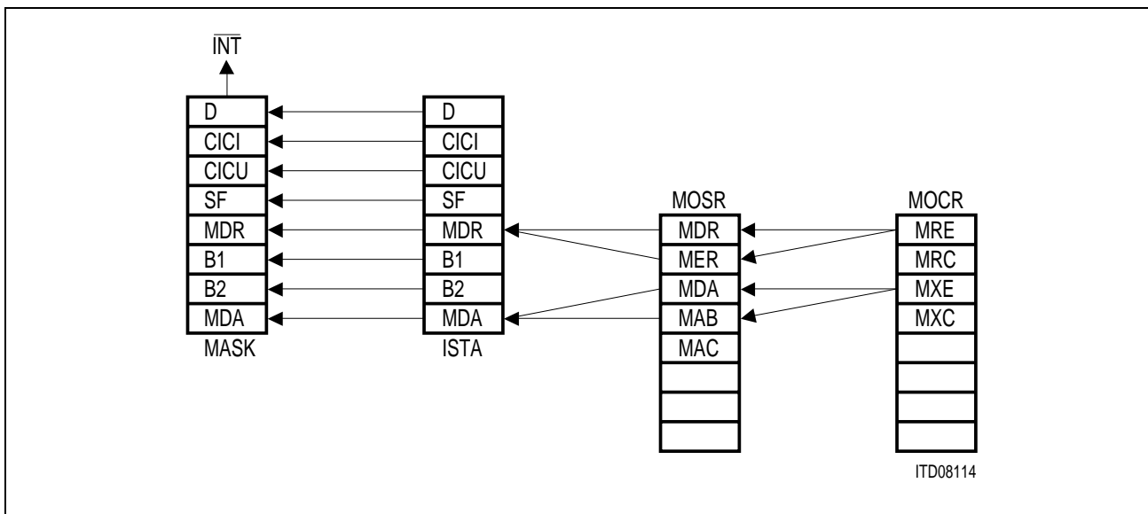
Figure 90 Interrupt Structure
