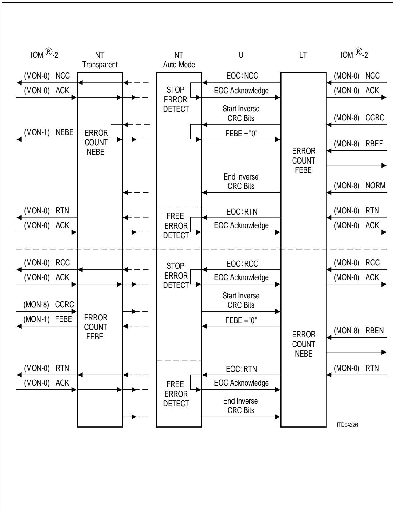
Figure 78 Block Error Counter Test
