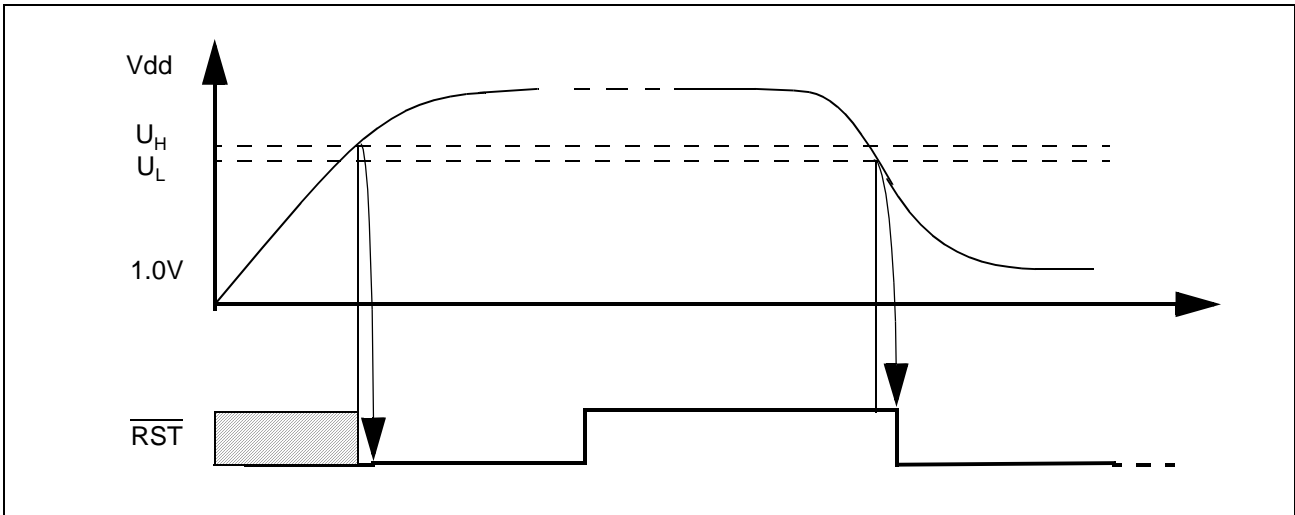
Figure 37 UVD Control of Pin RST
