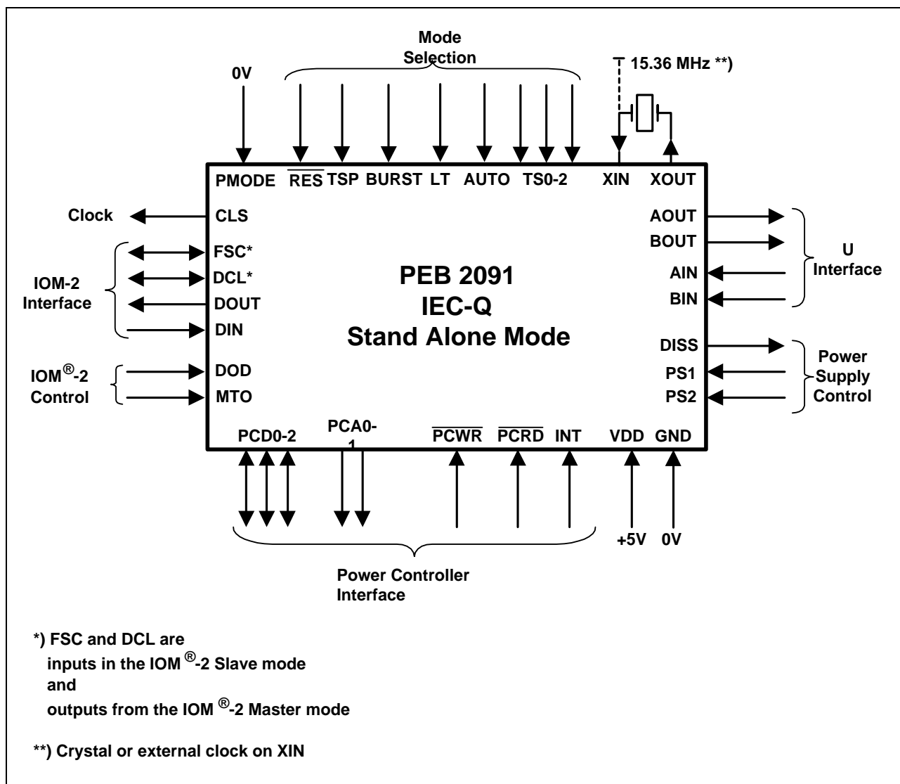
Figure 2 Logic Symbol for Stand-Alone Mode
