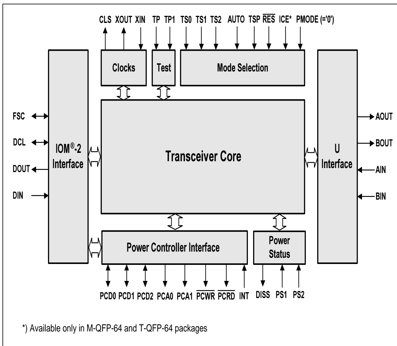
Figure 17 Device Architecture in Stand-Alone Mode
