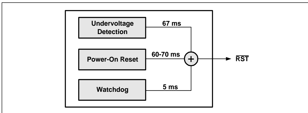
Figure 38 Reset Sources
