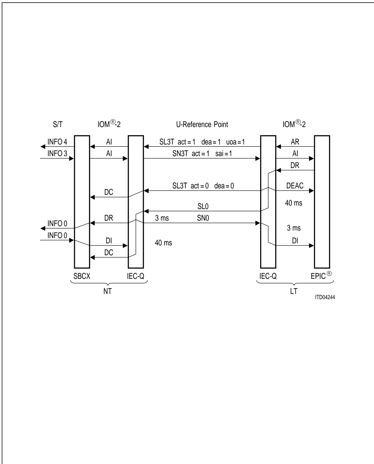
Figure 56 Complete Deactivation
