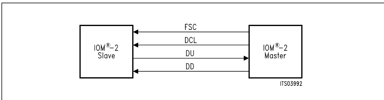
Figure 23 IOM ® -2 Clocks and Data Lines
