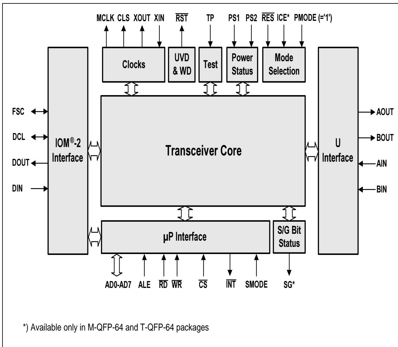
Figure 16 Device Architecture in μP Mode
