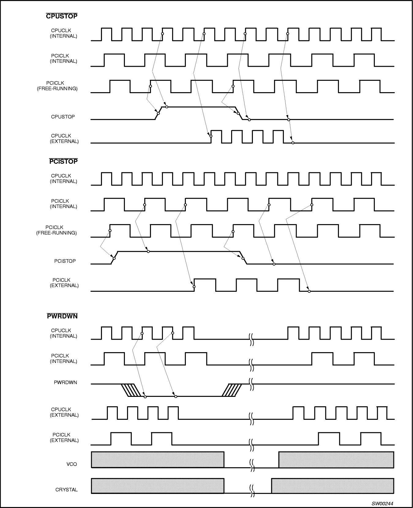
Figure 6. Power Management
