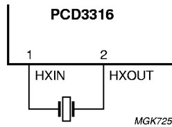
a. Standard oscillator: quartz or PXE.
