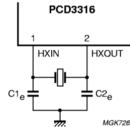
b. Oscillator: quartz or PXE with external capacitors.
