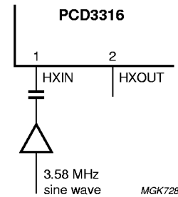
d. External clock: sine wave.
