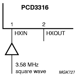
c. External clock: square wave.
