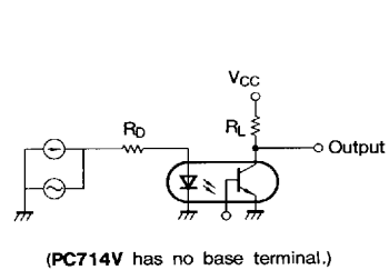
Test Circuit for Frequency Response
