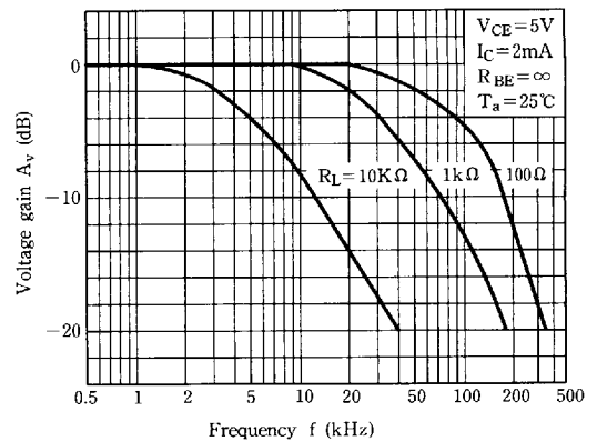
Fig.12 Frequency Response
