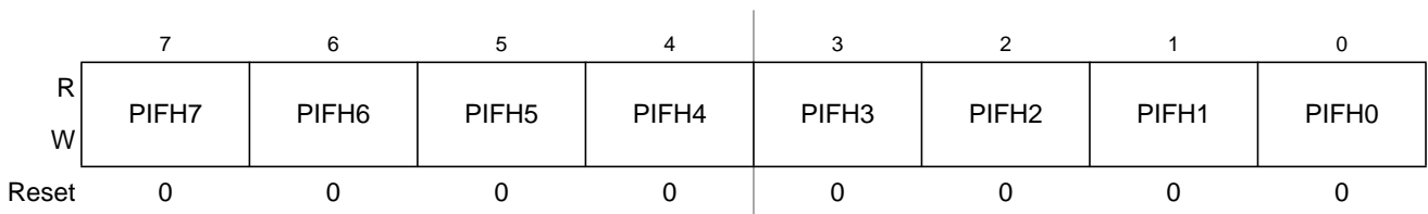
Figure 23-55. Port H Interrupt Flag Register (PIFH)
