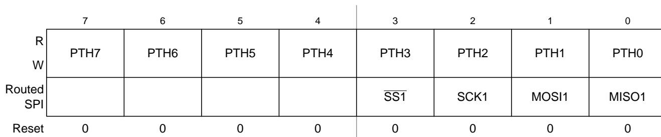
Figure 24-44. Port H Data Register (PTH)
