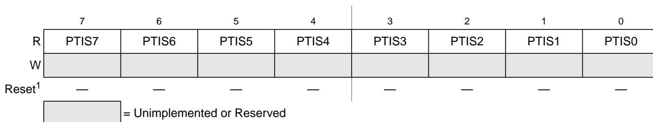
Figure 23-26. Port S Input Register (PTIS)
