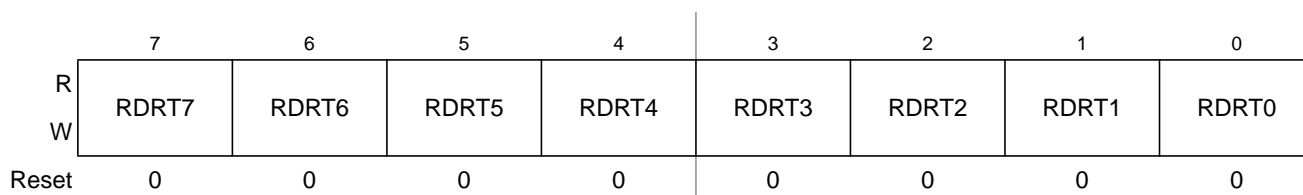
Figure 23-22. Port T Reduced Drive Register (RDRT)
