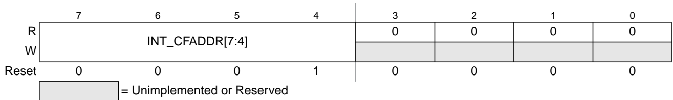
Figure 16-5. Interrupt Configuration Address Register (INT_CFADDR)
