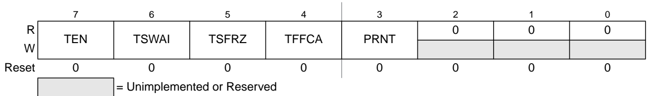
Figure 7-9. Timer System Control Register 1 (TSCR1)
