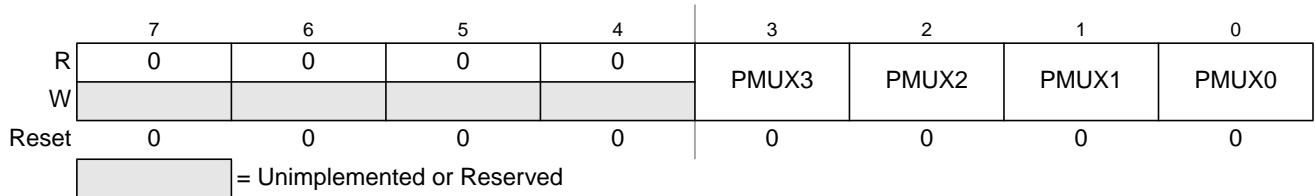
Figure 13-6. PIT Multiplex Register (PITMUX)
