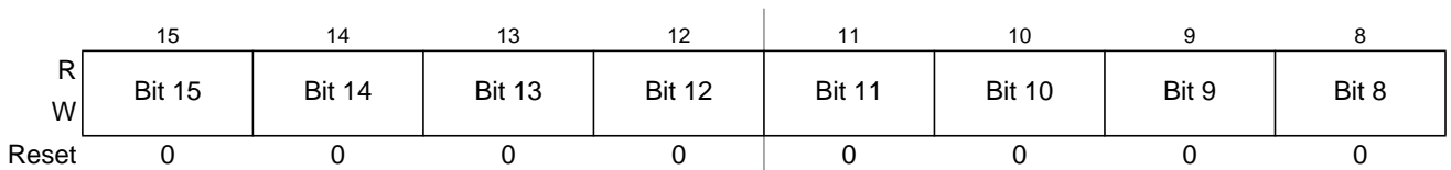
Figure 7-29. Timer Input Capture/Output Compare Register 5 High (TC5)
