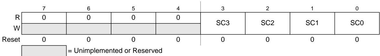
Figure 20-9. Debug State Control Register 1 (DBGSCR1)
