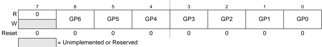
Figure 18-6. Global Page Index Register (GPAGE)
