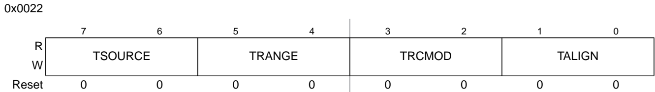
Figure 19-5. Debug Trace Control Register (DBGTCR)
