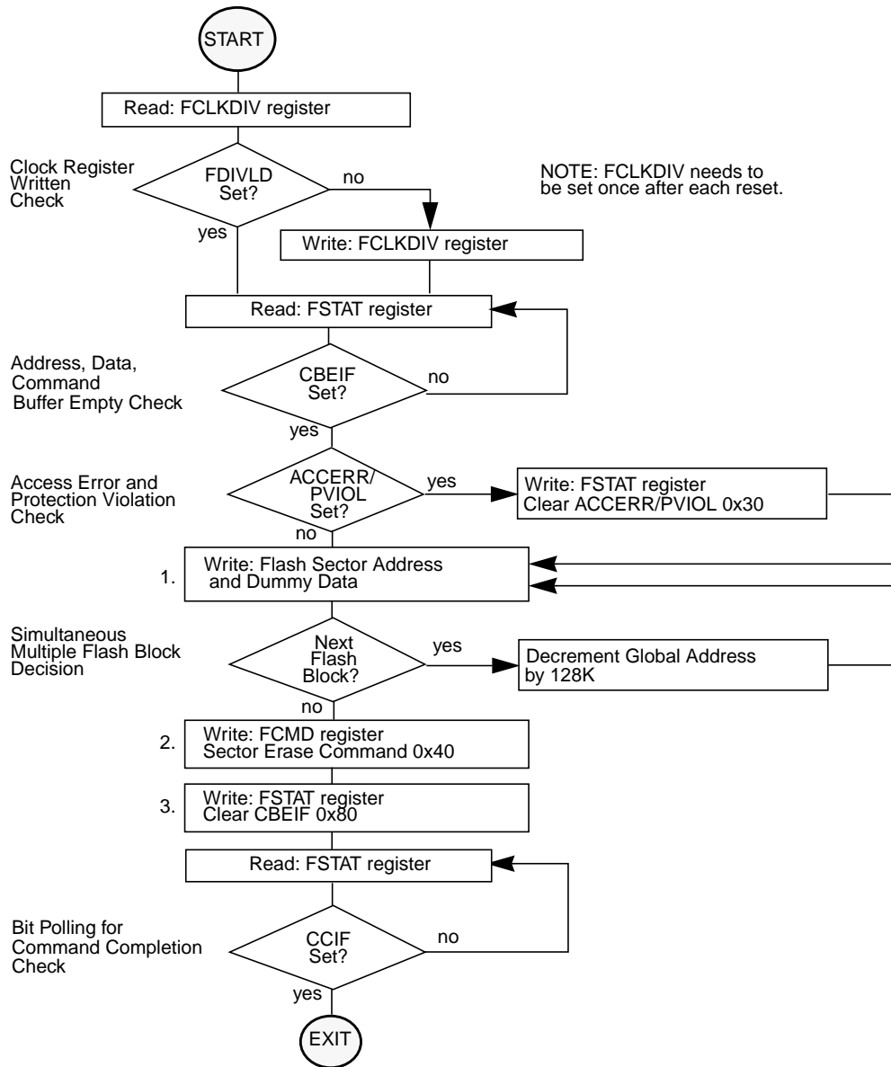
Figure 27-29. Example Sector Erase Command Flow
