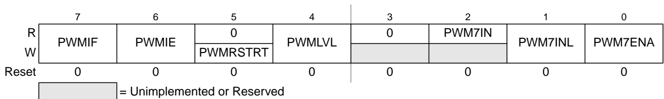
Figure 8-17. PWM Shutdown Register (PWMSDN)
