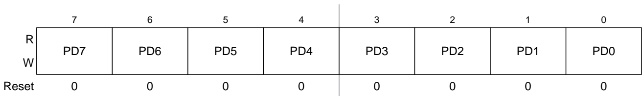
Figure 23-8. Port D Data Register (PORTD)
