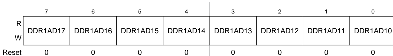
Figure 24-63. Port AD1 Data Direction Register 1 (DDR1AD1)
