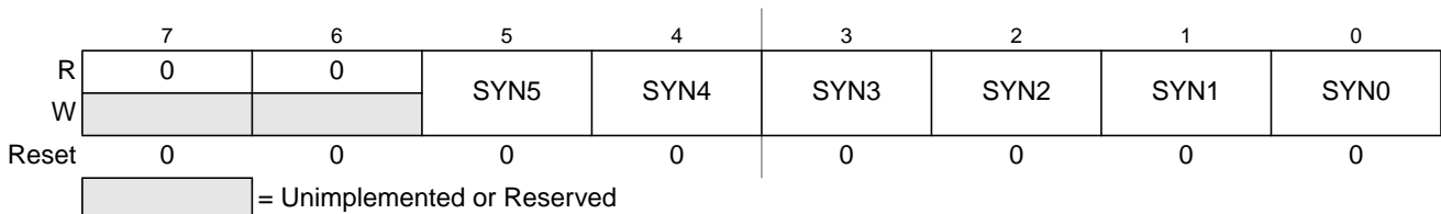
Figure 2-4. CRG Synthesizer Register (SYNR)
