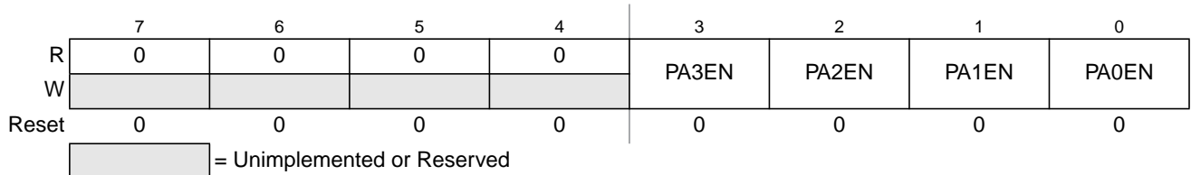
Figure 7-43. Input Control Pulse Accumulators Register (ICPAR)
