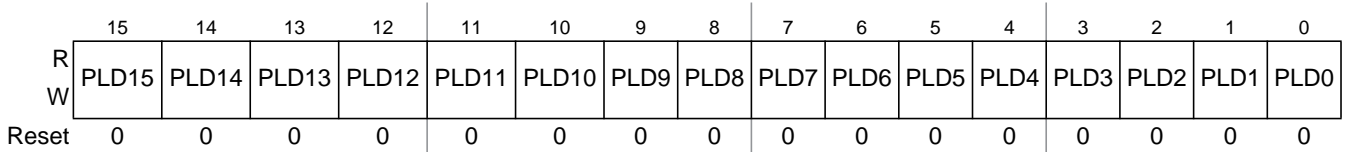
Figure 13-11. PIT Load Register 0 (PITLD0)
