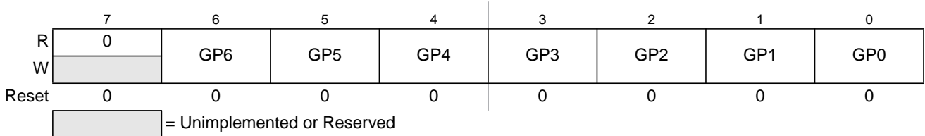
Figure 17-6. Global Page Index Register (GPAGE)
