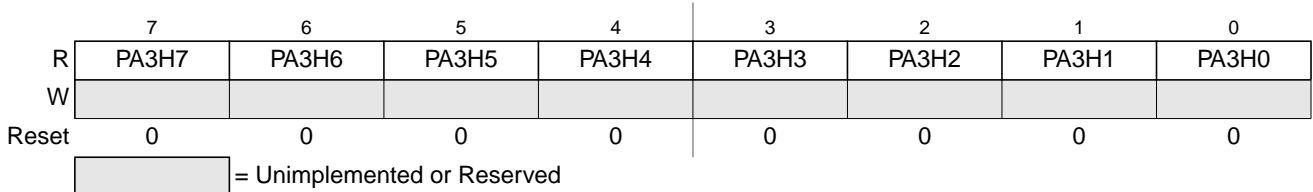
Figure 7-51. 8-Bit Pulse Accumulators Holding Register 3 (PA3H)
