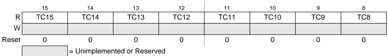
Figure 7-57. Timer Input Capture Holding Register 0 High (TC0H)
