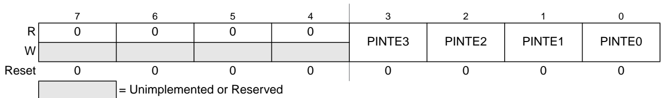
Figure 13-7. PIT Interrupt Enable Register (PITINTE)
