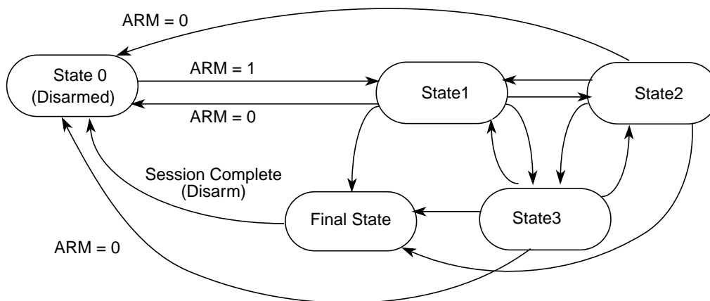
Figure 20-23. State Sequencer Diagram
