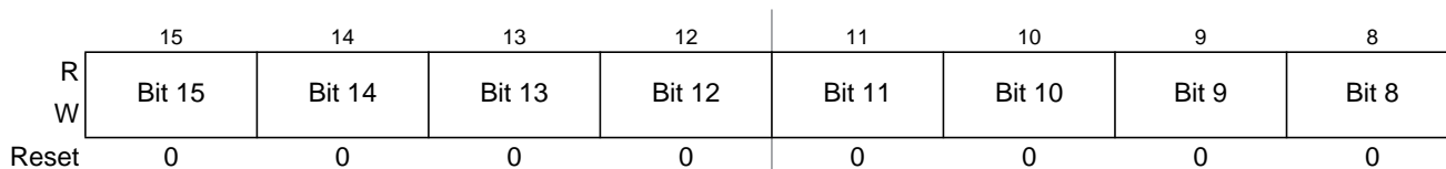
Figure 7-19. Timer Input Capture/Output Compare Register 0 High (TC0)
