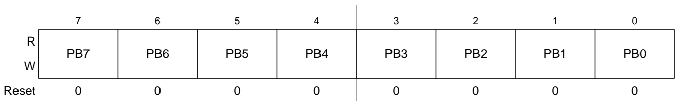
Figure 24-4. Port B Data Register (PORTB)
