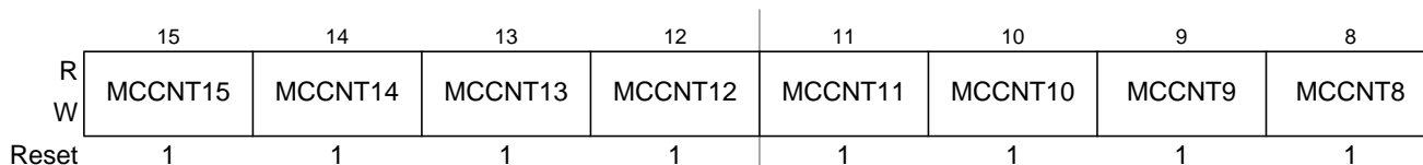
Figure 7-55. Modulus Down-Counter Count Register High (MCCNT)
