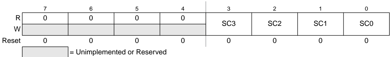
Figure 20-11. Debug State Control Register 3 (DBGSCR3)
