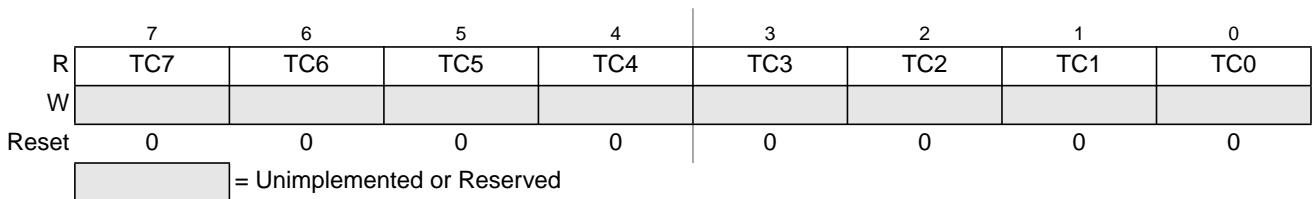
Figure 7-58. Timer Input Capture Holding Register 0 Low (TC0L)
