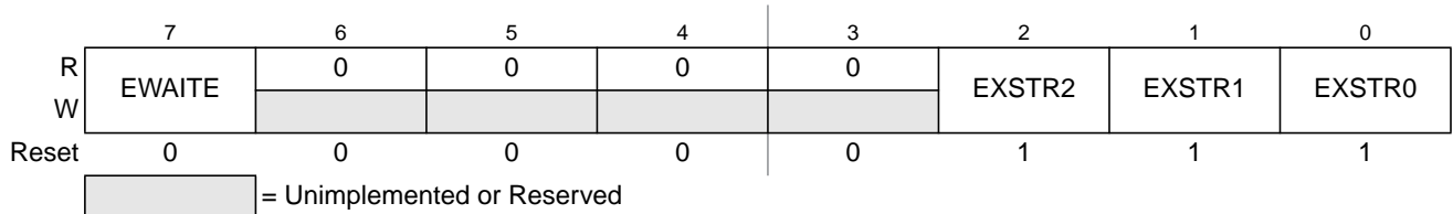
Figure 21-4. External Bus Interface Control Register 1 (EBICTL1)
