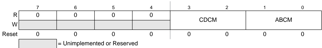
Figure 20-6. Debug Control Register2 (DBGC2)
