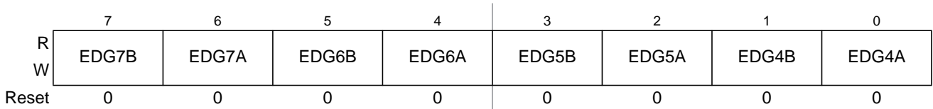
Figure 7-13. Timer Control Register 3 (TCTL3)
