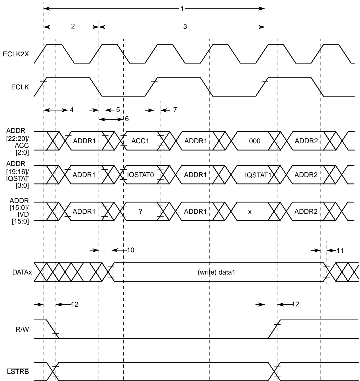
Figure A-16. Example 2b: Emulation Expanded Mode Write with 1 Stretch Cycle
