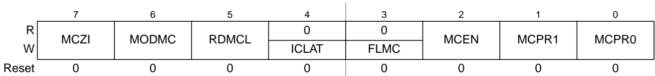
Figure 7-41. 16-Bit Modulus Down-Counter Control Register (MCCTL)
