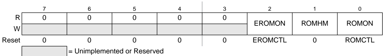
Figure 17-10. MMC Control Register (MMCCTL1)
