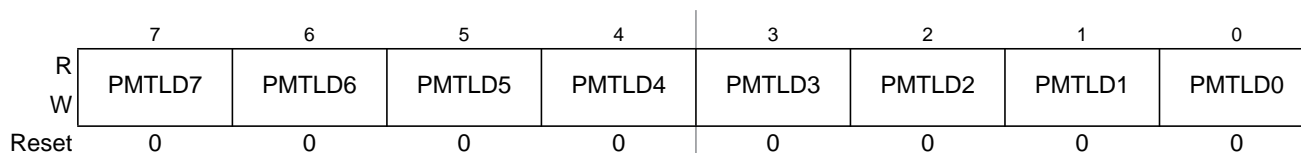
Figure 13-9. PIT Micro Timer Load Register 0 (PITMTLD0)
