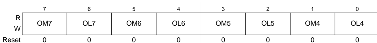
Figure 7-11. Timer Control Register 1 (TCTL1)
