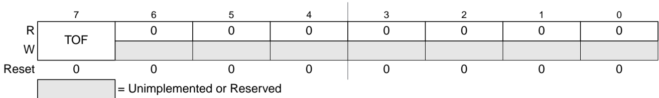
Figure 7-18. Main Timer Interrupt Flag 2 (TFLG2)
