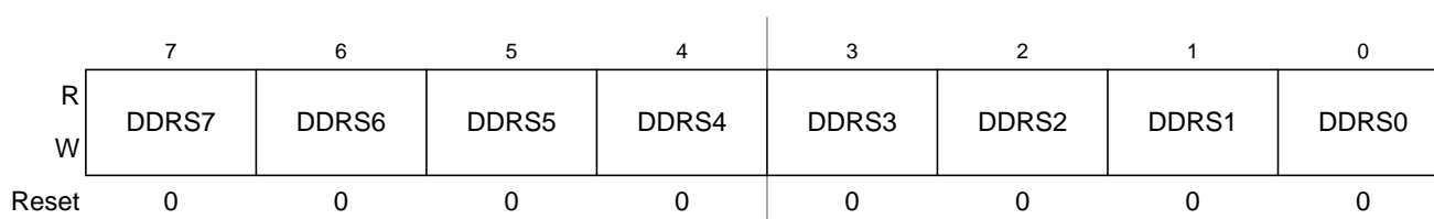
Figure 23-27. Port S Data Direction Register (DDRS)
