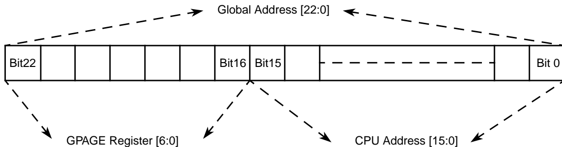
Figure 17-7. GPAGE Address Mapping
