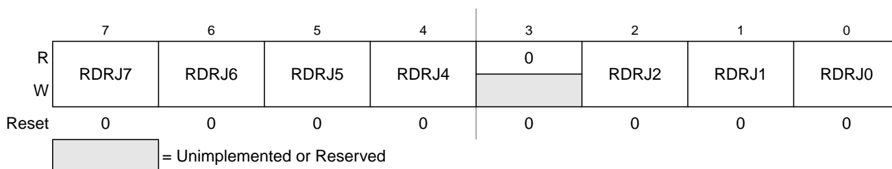
Figure 23-59. Port J Reduced Drive Register (RDRJ)
