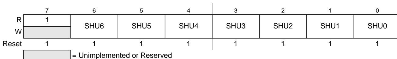
Figure 17-20. RAM Shared Region Upper Boundary Register (RAMSHU)
