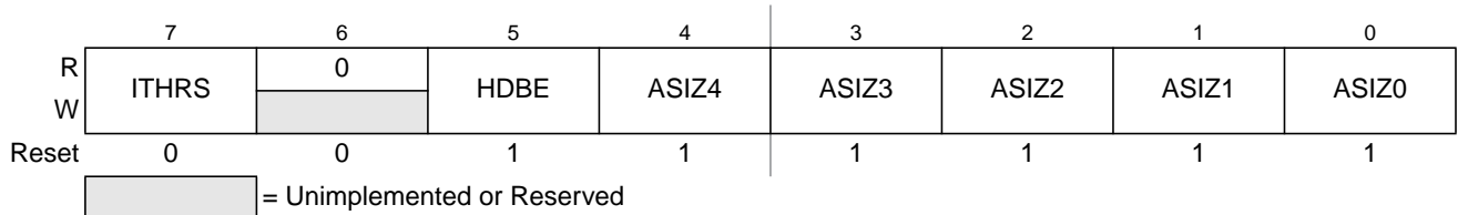
Figure 21-3. External Bus Interface Control Register 0 (EBICTL0)
