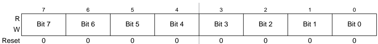
Figure 7-30. Timer Input Capture/Output Compare Register 5 Low (TC5)
