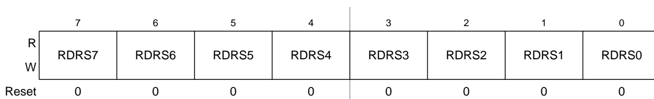
Figure 23-28. Port S Reduced Drive Register (RDRS)
