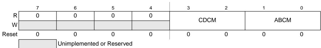
Figure 19-6. Debug Control Register2 (DBG2)
