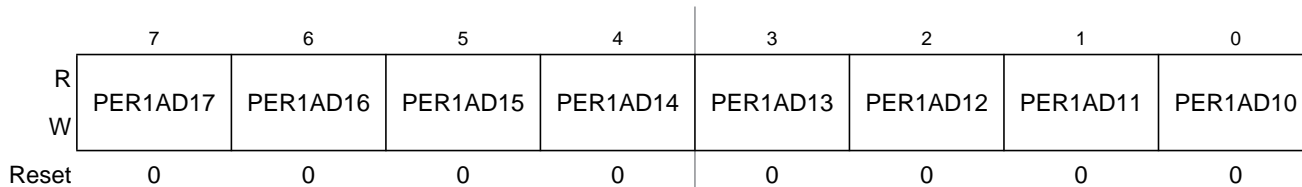
Figure 24-67. Port AD1 Pull Up Enable Register 1 (PER1AD1)
