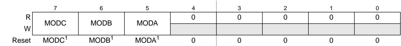
Figure 17-4. Mode Register (MODE)
