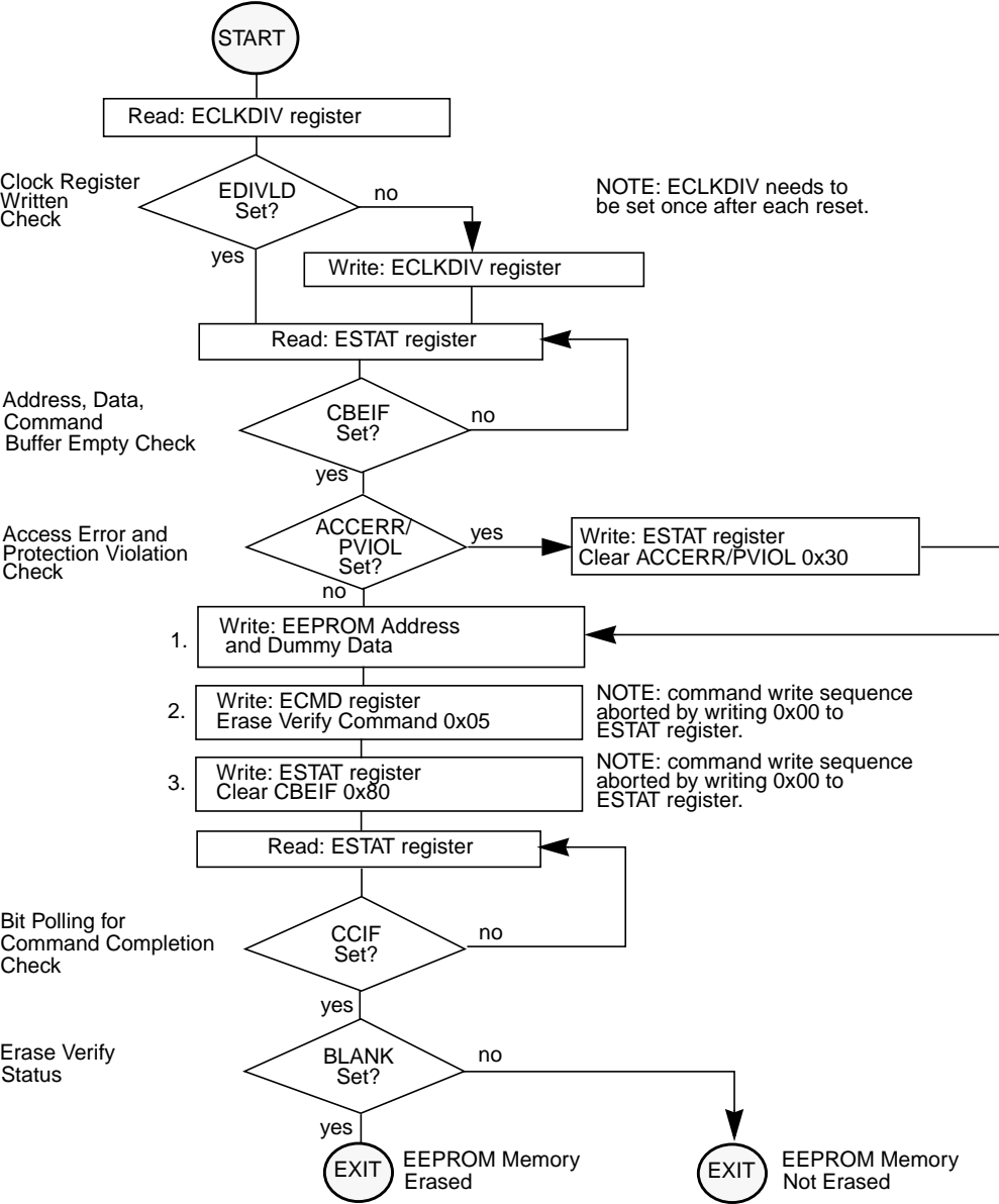
Figure 25-18. Example Erase Verify Command Flow
