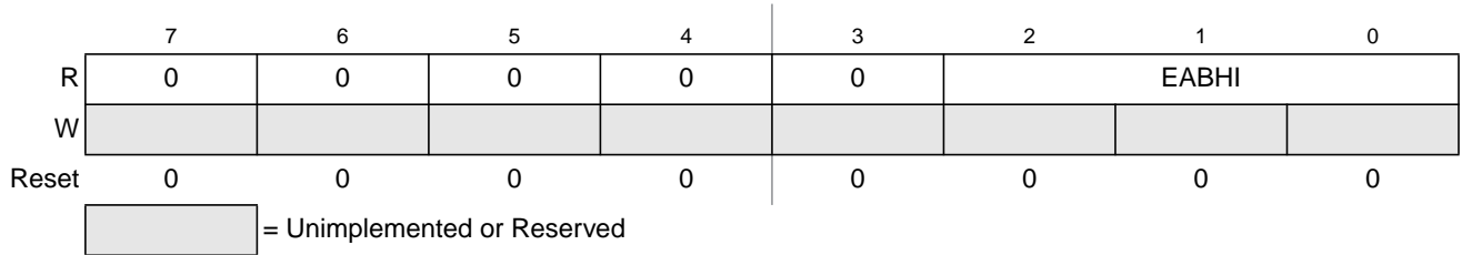
Figure 26-13. EEPROM Address High Register (EADDRHI)
