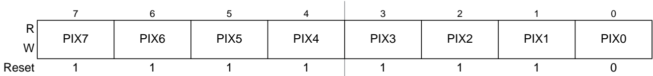
Figure 18-15. Program Page Index Register (PPAGE)
