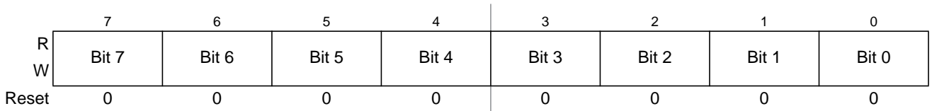
Figure 7-26. Timer Input Capture/Output Compare Register 3 Low (TC3)
