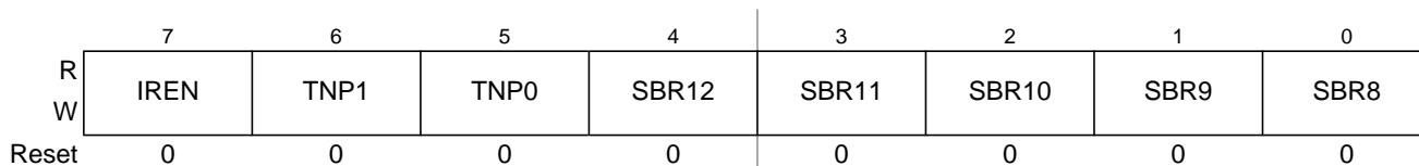
Figure 11-3. SCI Baud Rate Register (SCIBDH)
