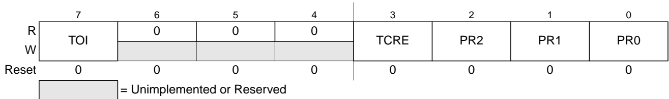
Figure 7-16. Timer System Control Register 2 (TSCR2)
