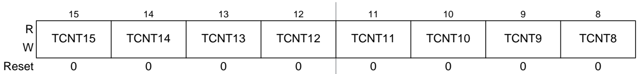
Figure 7-7. Timer Count Register High (TCNT)
