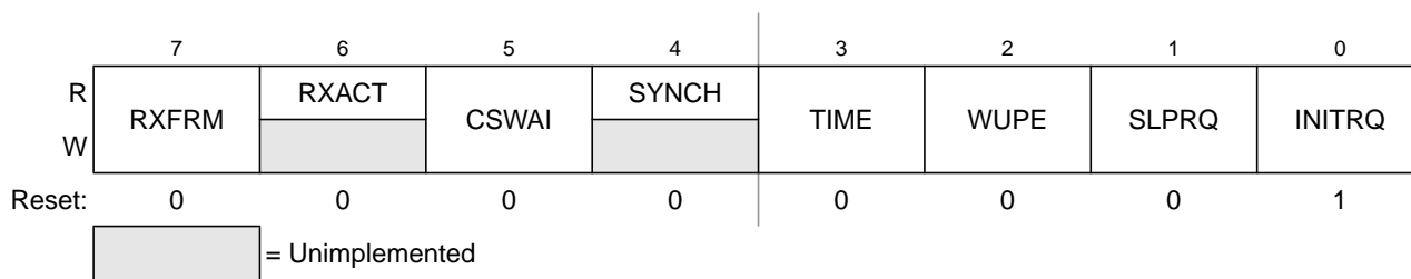
Figure 10-4. MSCAN Control Register 0 (CANCTL0)
