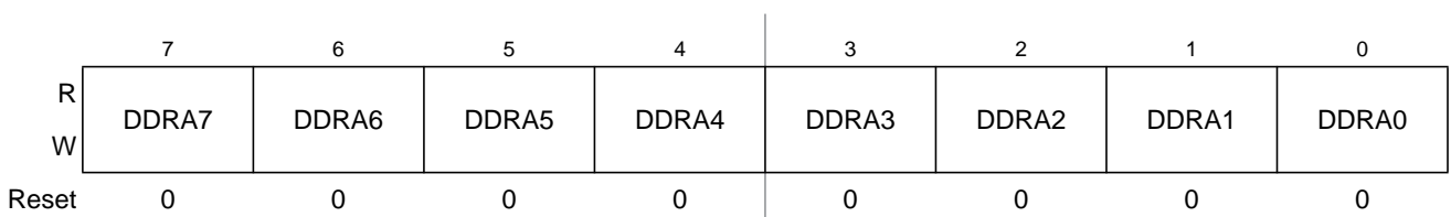
Figure 23-5. Port A Data Direction Register (DDRA)
