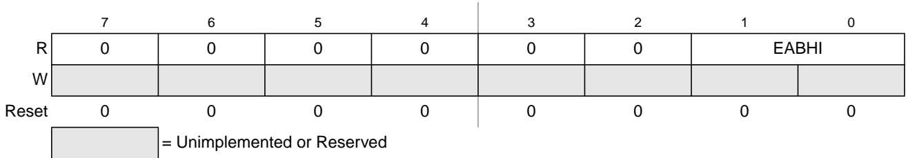
Figure 25-13. EEPROM Address High Register (EADDRHI)
