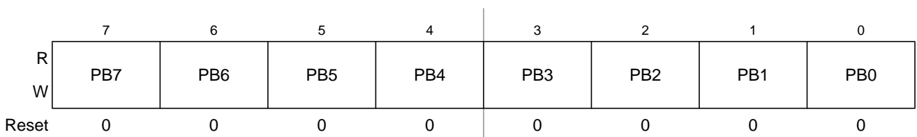
Figure 23-4. Port B Data Register (PORTB)
