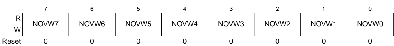
Figure 7-45. Input Control Overwrite Register (ICOVW)
