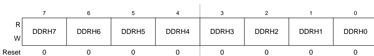
Figure 23-50. Port H Data Direction Register (DDRH)
