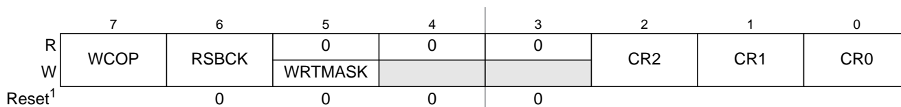
Figure 2-12. CRG COP Control Register (COPCTL)
