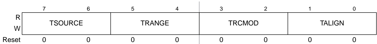
Figure 20-5. Debug Trace Control Register (DBGTCR)
