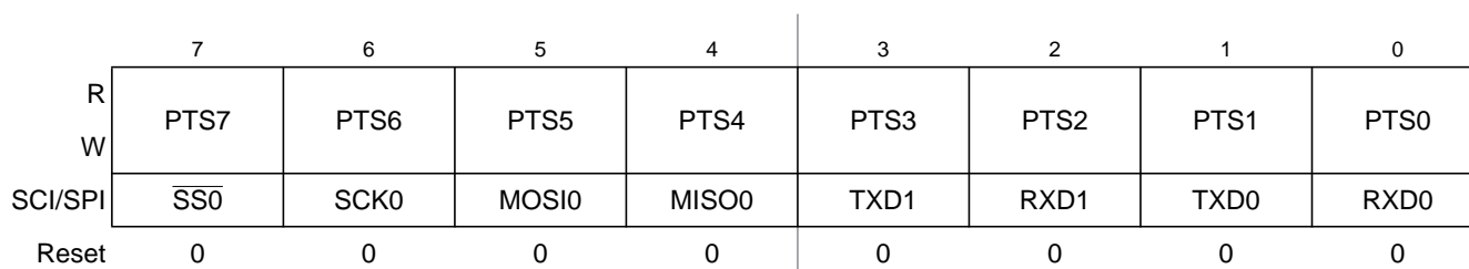
Figure 23-25. Port S Data Register (PTS)
