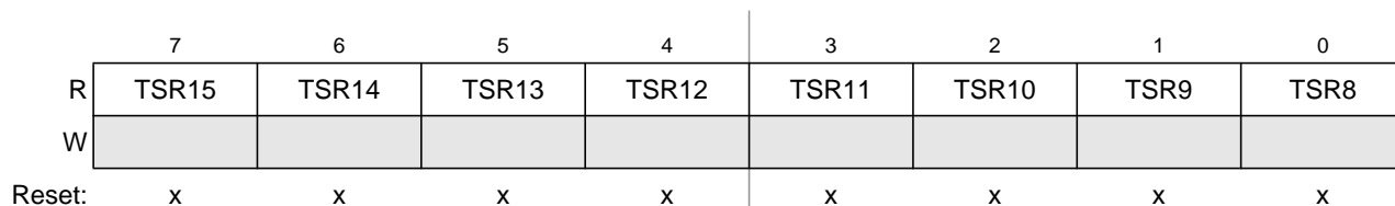
Figure 10-37. Time Stamp Register — High Byte (TSRH)
