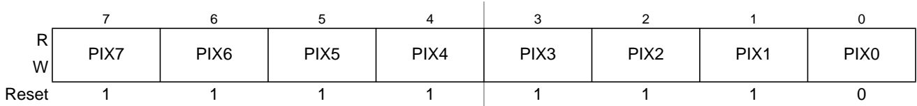
Figure 17-15. Program Page Index Register (PPAGE)
