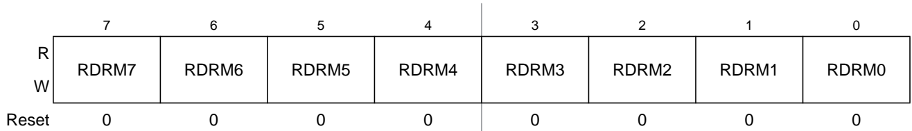
Figure 23-35. Port M Reduced Drive Register (RDRM)
