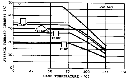
FIG.3-AVERAGE FORWARD CURRENT VS. CASE TEMPERATURE
