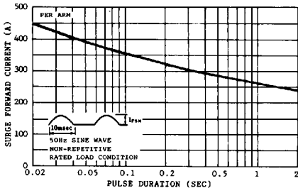
FIG.4-SURGE CURRENT RATINGS
