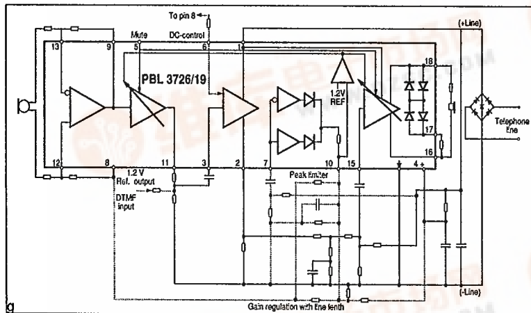
Figure 1. Functional diagram.
