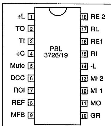
Figure 5. Pin configuration.
