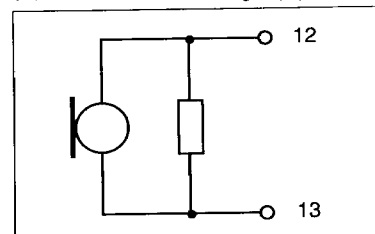
Figure 16. Connection of a magnetic microphone.
