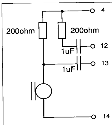
Figure 14. Electret microphone with FET-buffer, e.g. EM80.
