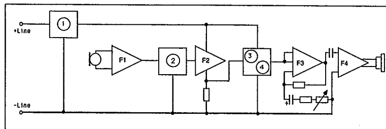
Figure 7. Alternative block interconnections.
