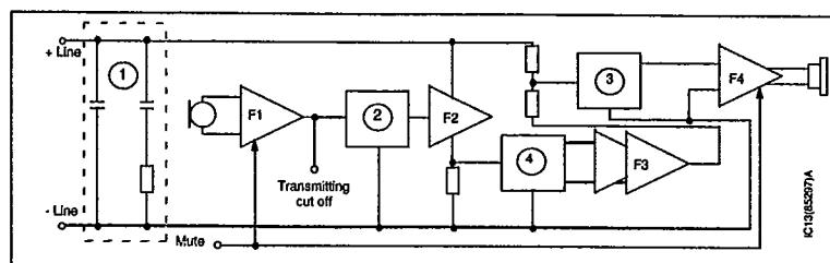
Figure 6. Block interconnections.
