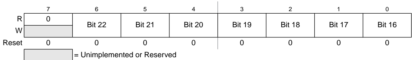
Figure 20-15. Debug Comparator Address High Register (DBGXAH)
