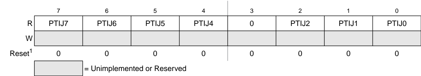
Figure 22-57. Port J Input Register (PTIJ)
