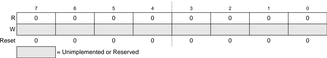
Figure 25-12. RESERVED3
