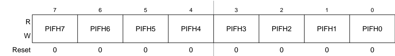
Figure 22-55. Port H Interrupt Flag Register (PIFH)
