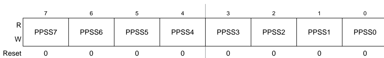
Figure 24-26. Port S Polarity Select Register (PPSS)
