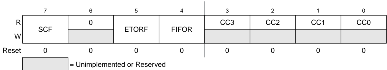
Figure 4-9. ATD Status Register 0 (ATDSTAT0)
