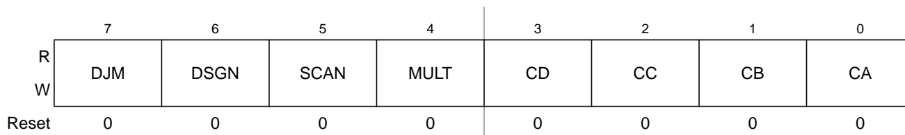
Figure 4-8. ATD Control Register 5 (ATDCTL5)
