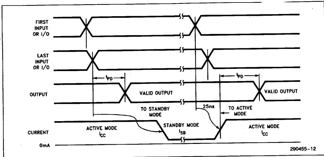
Figure 6. iPLD610 Standby and Active Mode Transitions
