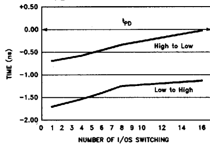
IPLD610 t_{PD} vs No. of Outputs Switching
