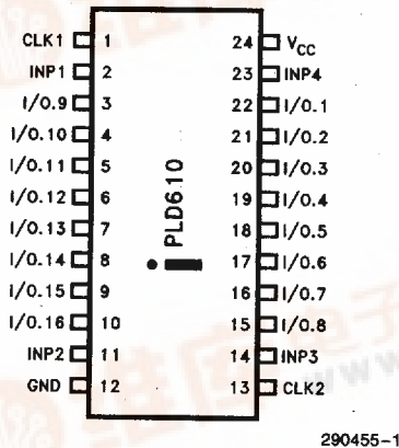
Figure 1. iPLD610 Pin Configurations
